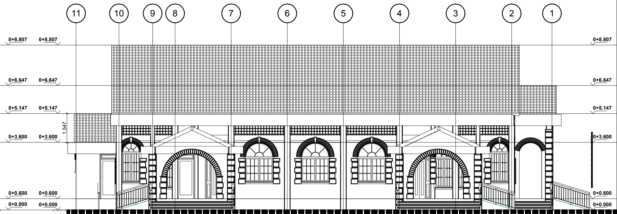
SIDE ELEVATION 04
