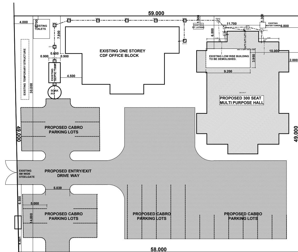
SITE BLOCK PLAN SCALE 1:400
