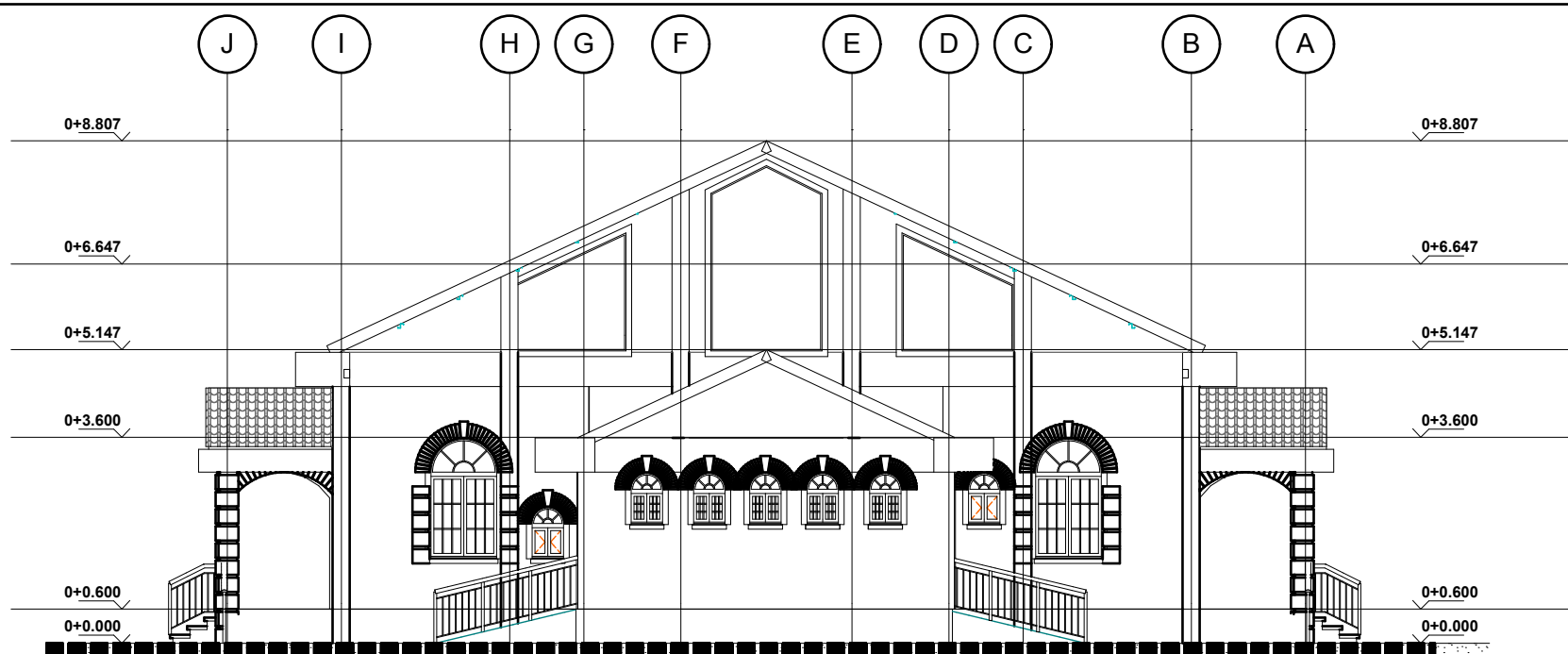
BACK ELEVATION 03
