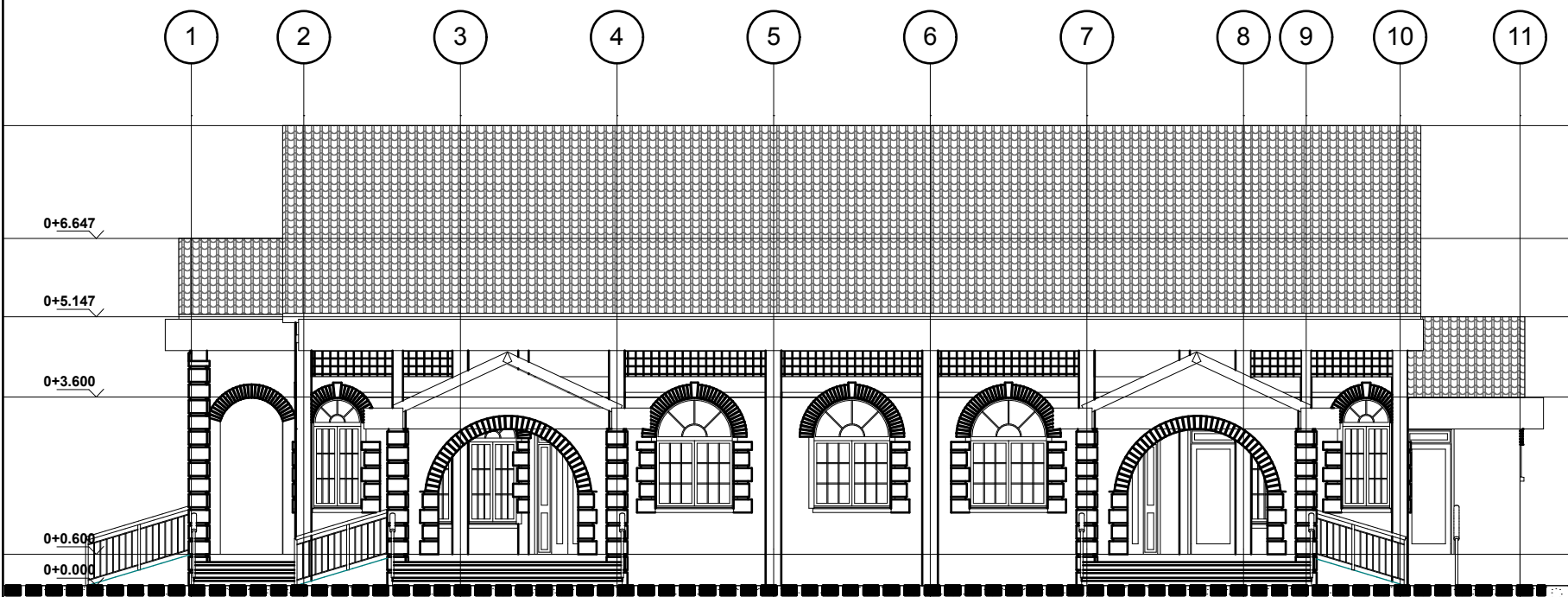
SIDE ELEVATION 02
