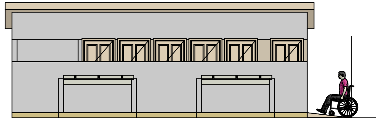
ELEVATION E-01
