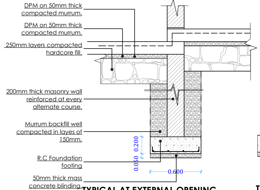
TYPICAL AT EXTERNAL OPENING FOUNDATION WALLS SCALE 1:25
