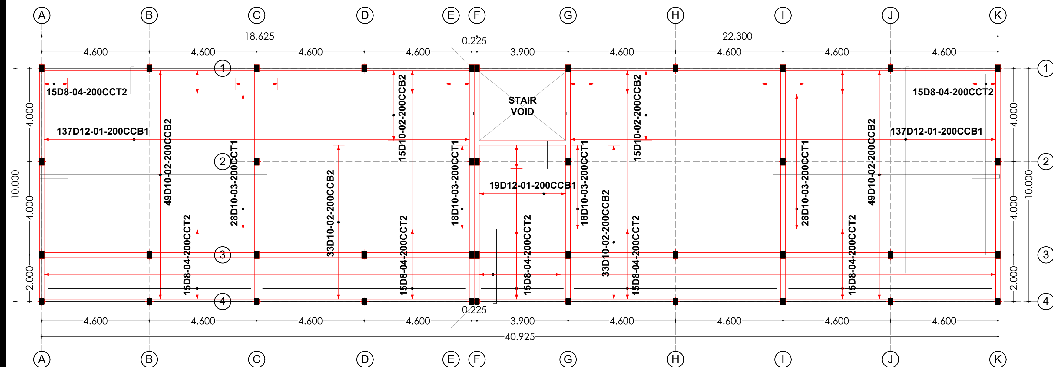
BAR ARRANGEMENT LAYOUT PLAN
