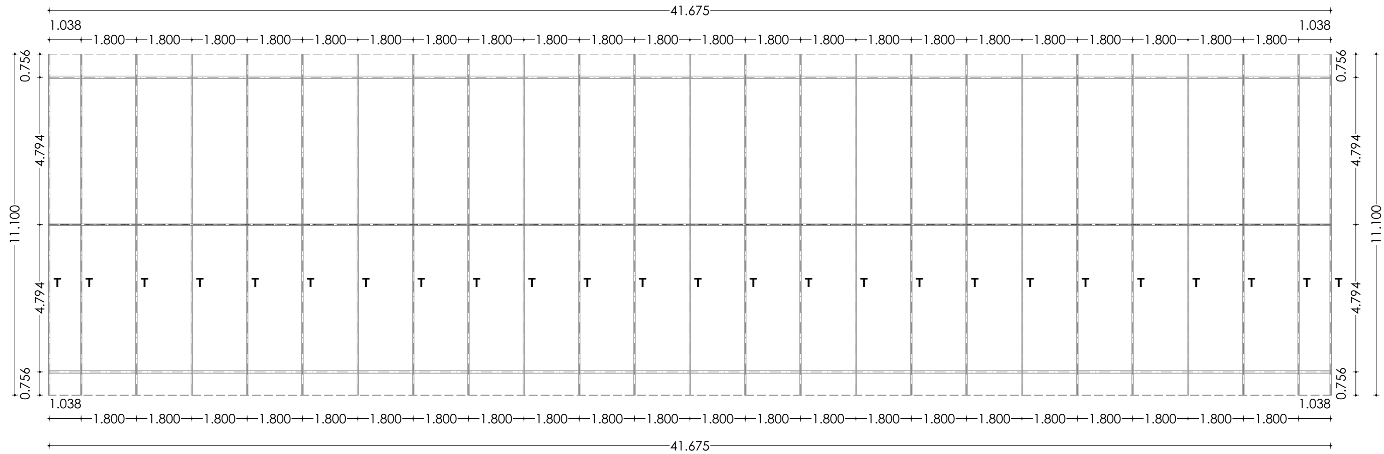
TRUSS LAYOUT PLAN
