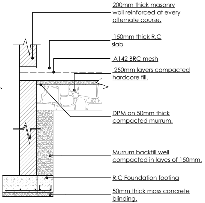
TYPICAL EXTERNAL FOUNDATION WALLS SCALE 1:25
