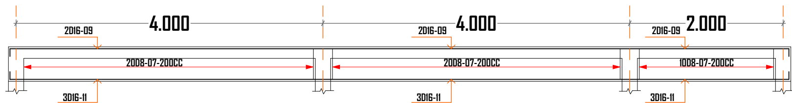
BEAM GRID A-A -[600 X200] SCALE 1:25
