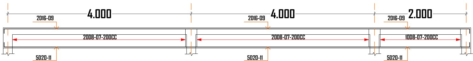
BEAM GRID B-B -[600 X200] SCALE 1:25
