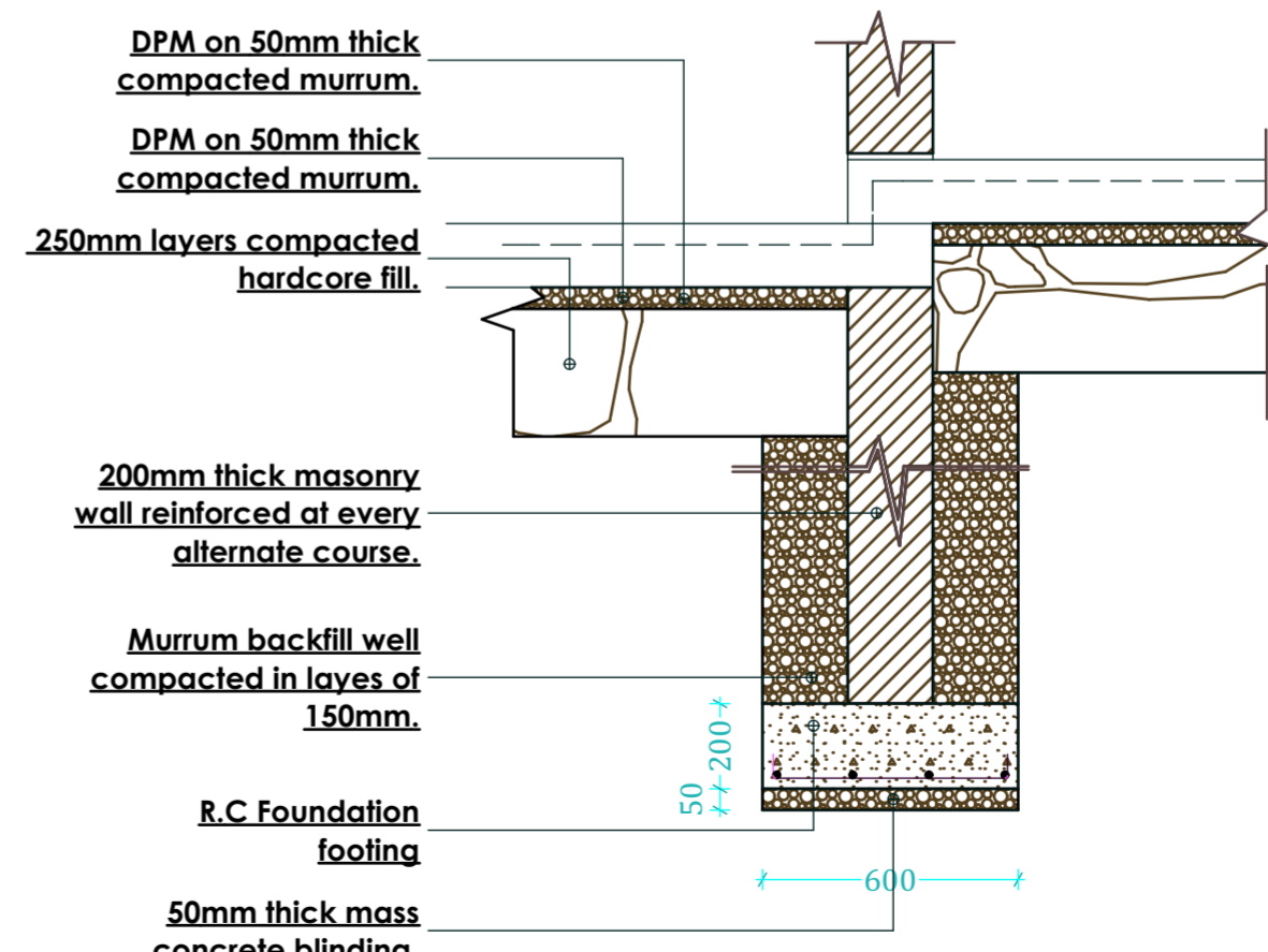
TYPICAL AT EXTERNAL OPENING FOUNDATION WALLS SCALE 1:25
