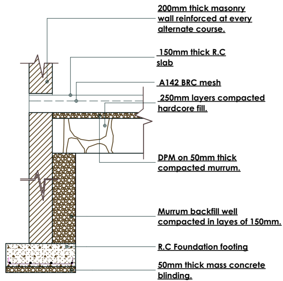
TYPICAL EXTERNAL FOUNDATION WALLS SCALE 1:25
