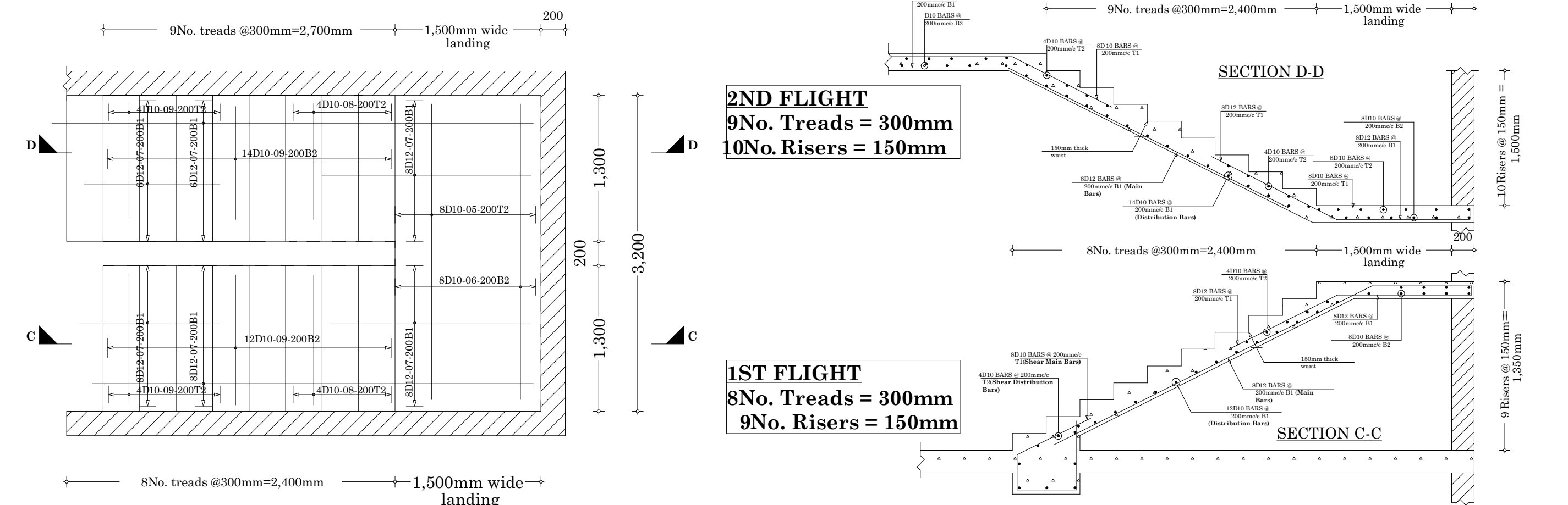
STAIR SECTIONS (1:50)
