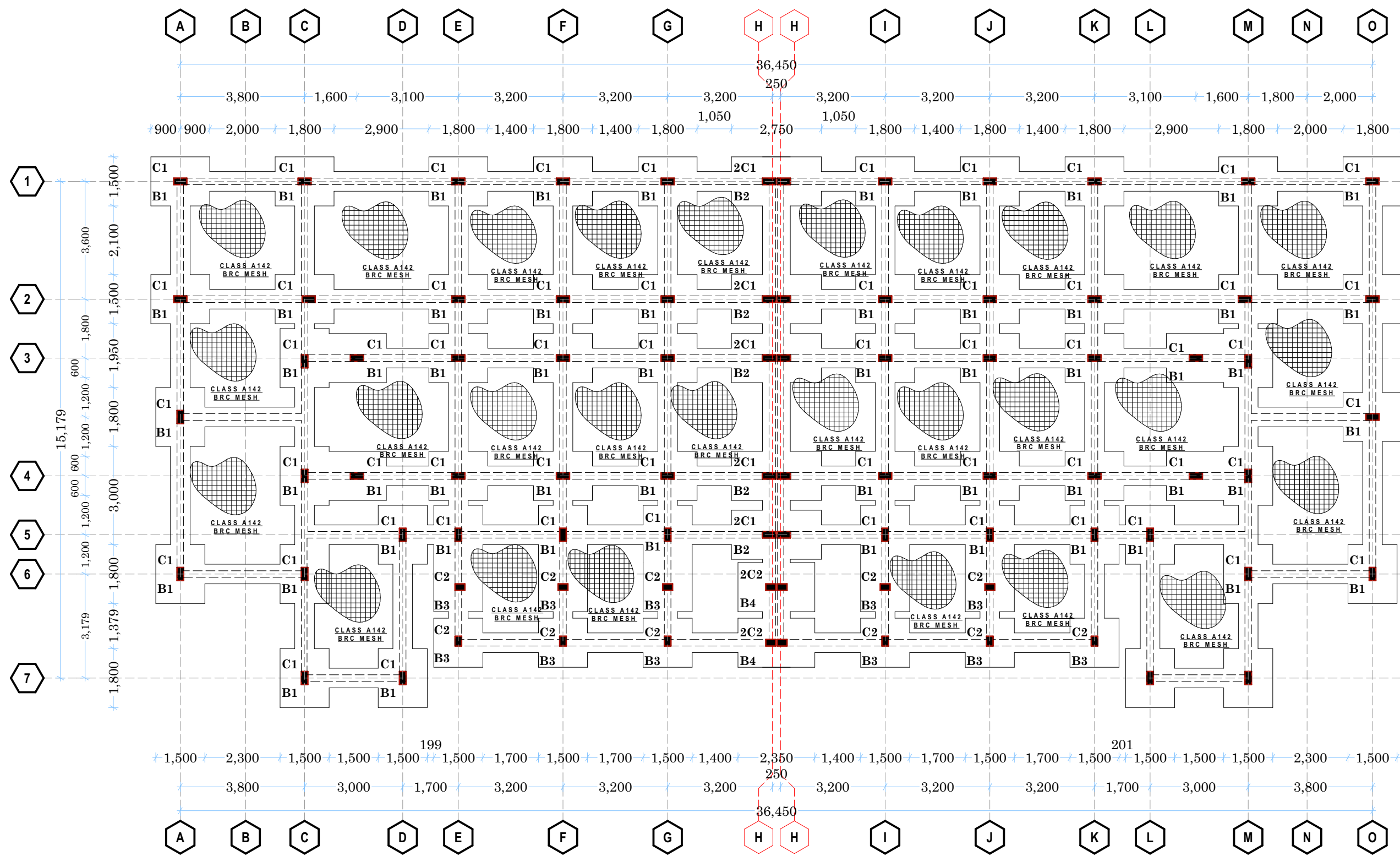
FOUNDATION LAYOUT COLUMN BASES & STRIP FDN SCALE 1:100
