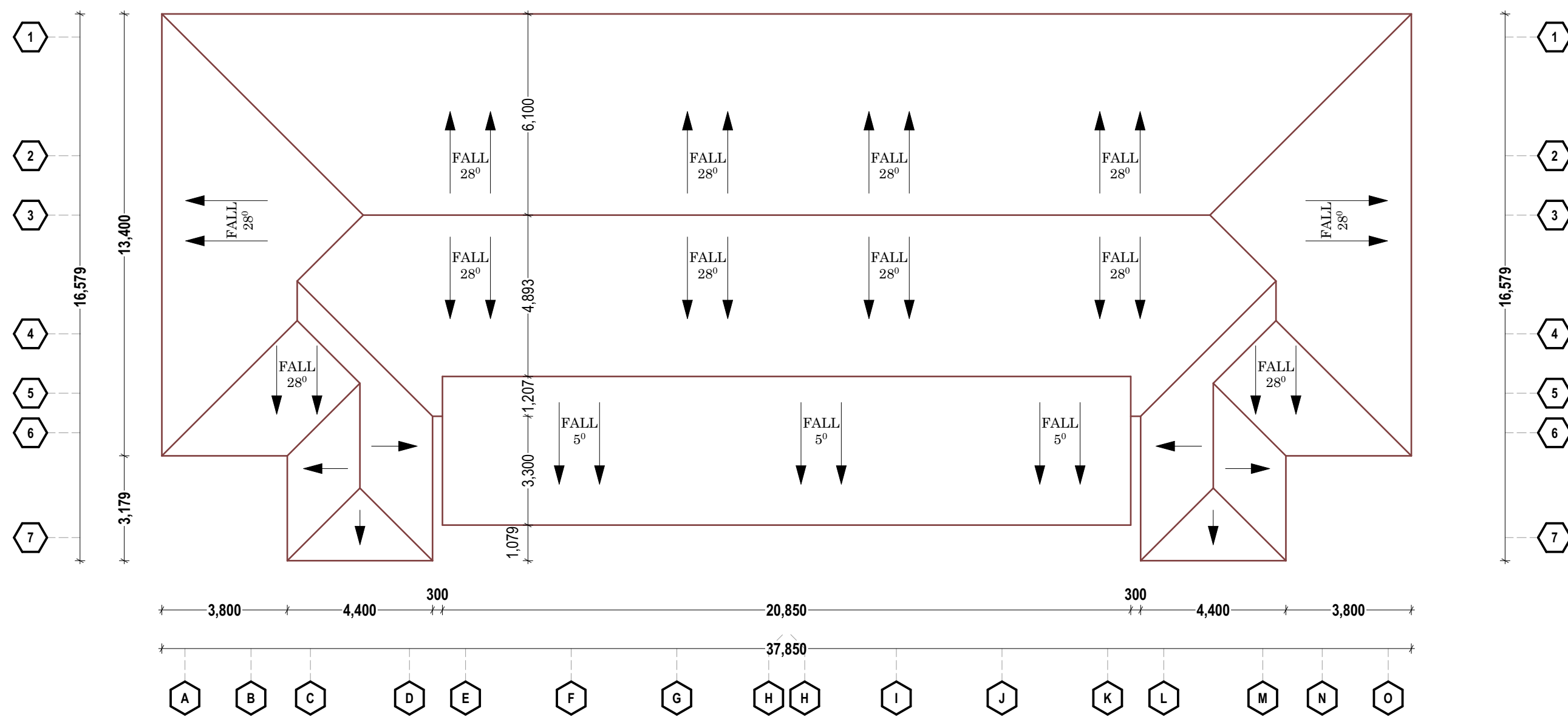
ROOF PLAN LAYOUT SCALE 1:100
