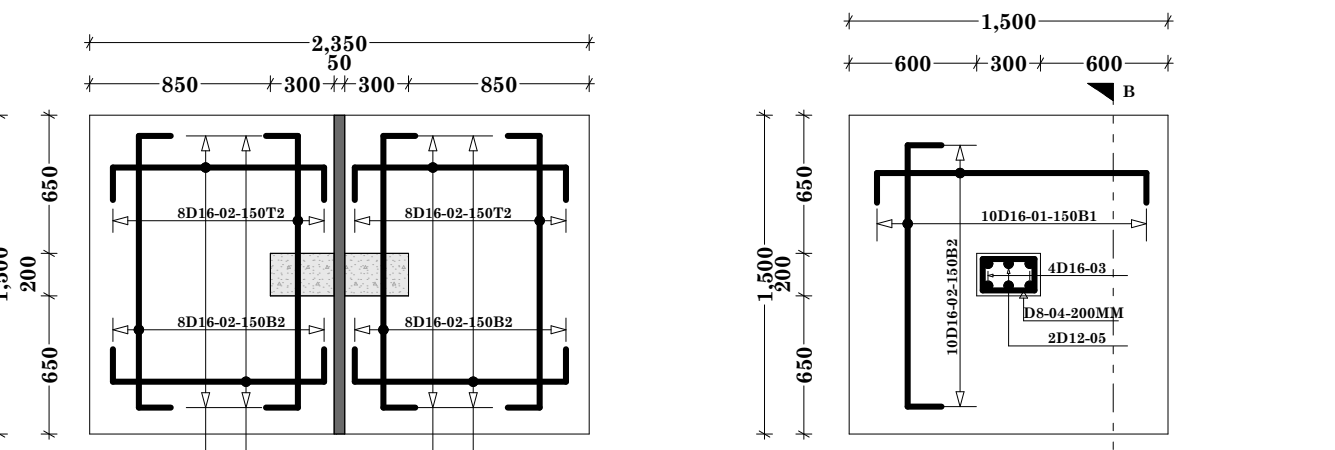
COLUMN C2-B3 BASE DETAILS SCALE 1:25
