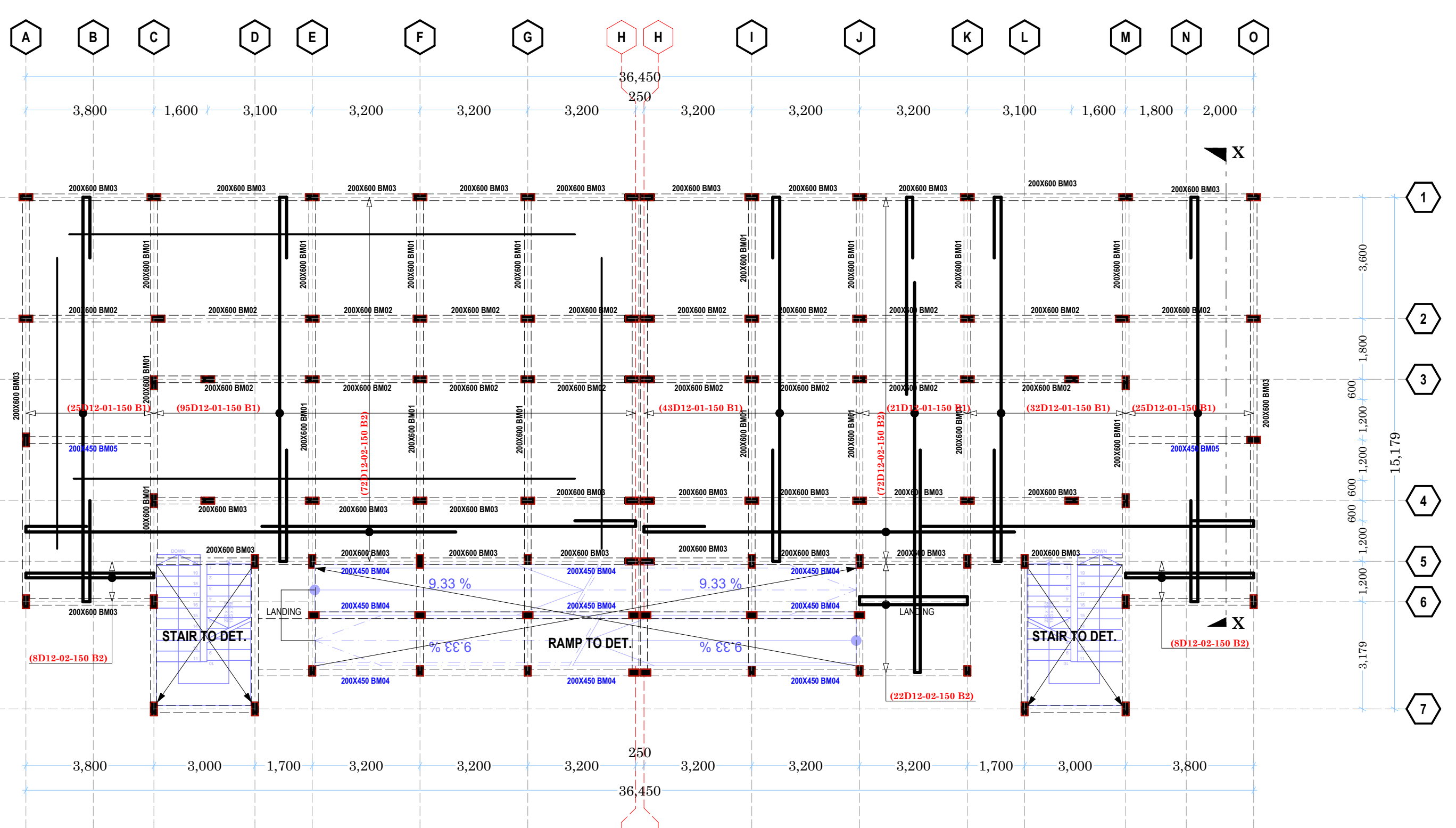
SUSPENDED SLAB REINFORCEMENT DETAILS SCALE 1:100
