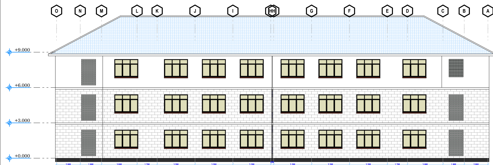
ELEVATION E-01 SCALE 1:100
