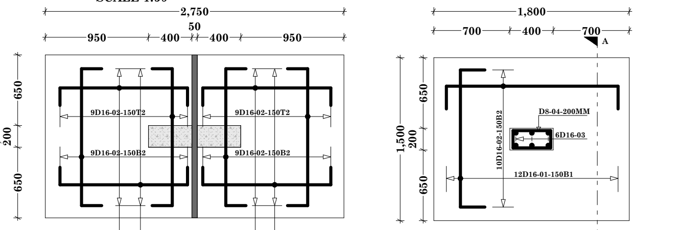
COLUMN C1-B1 BASE DETAILS SCALE 1:25
