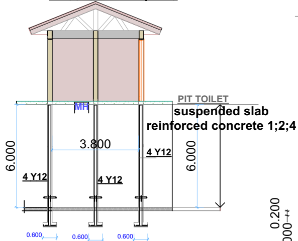
FRONT ELEVATIONS
