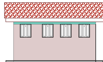
BACK ELEVATIONS
