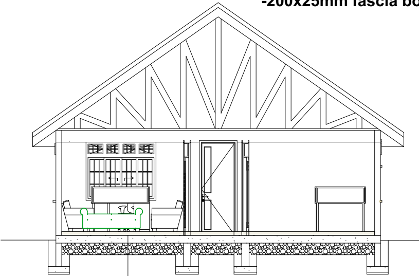
SECTION 02-02
