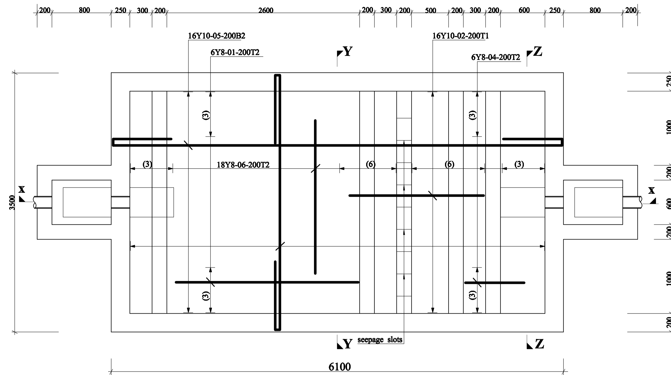
SEPTIC TANK PLAN
