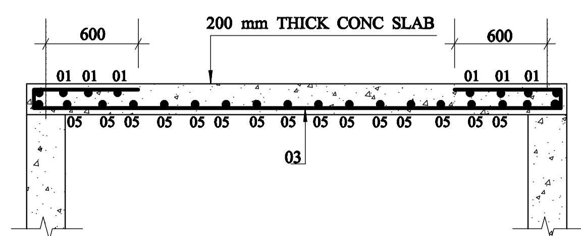
SECTION Y-Y
