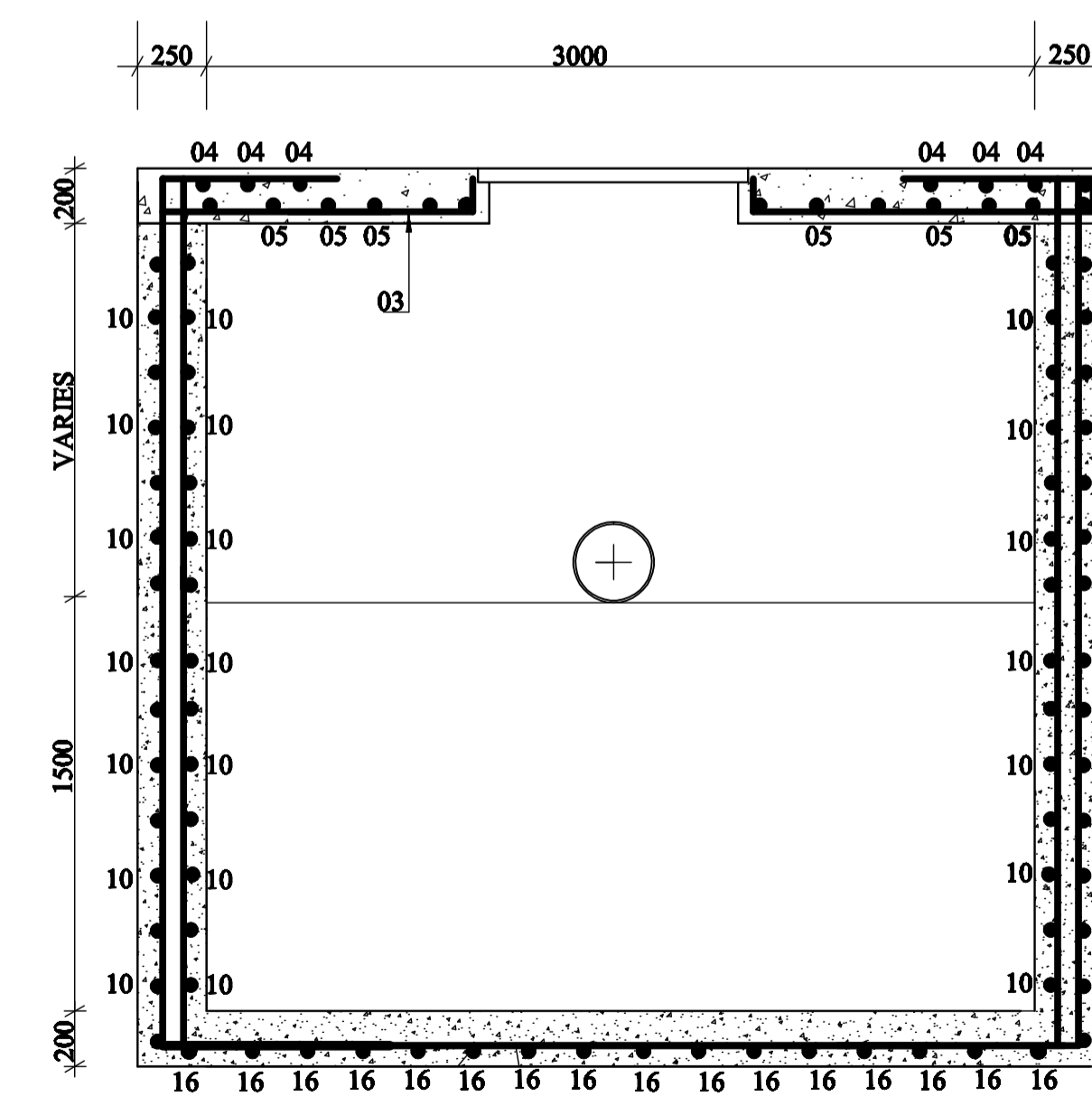
SECTION Z-Z
