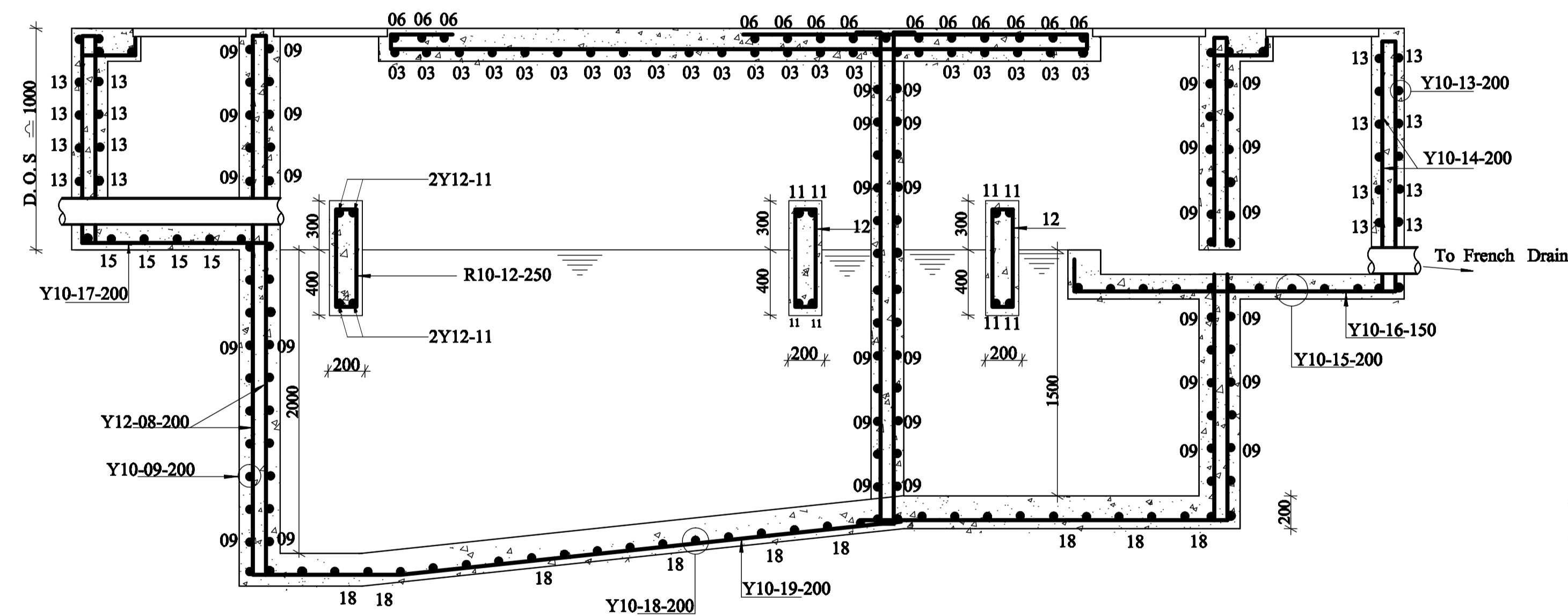
SECTION X-X
