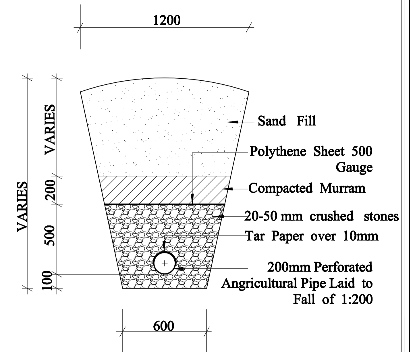
SECTION OF THE FRENCH DRAIN
