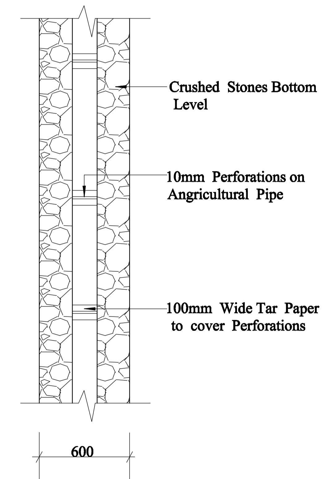
FRENCH DRAIN PLAN (LENGTH TO BE DETERMINED ON SITE)
