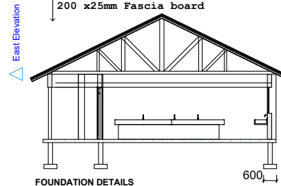
FOUNDATION DETAILS
