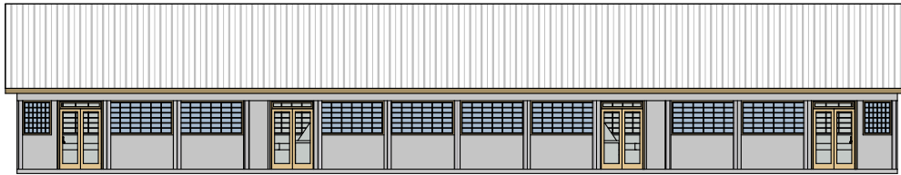
ELEVATION-01
