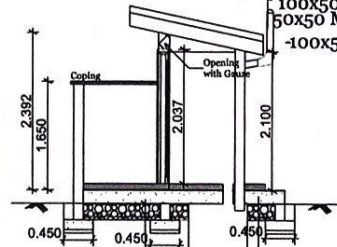
SECTION 02-02 SCALE 1:100
