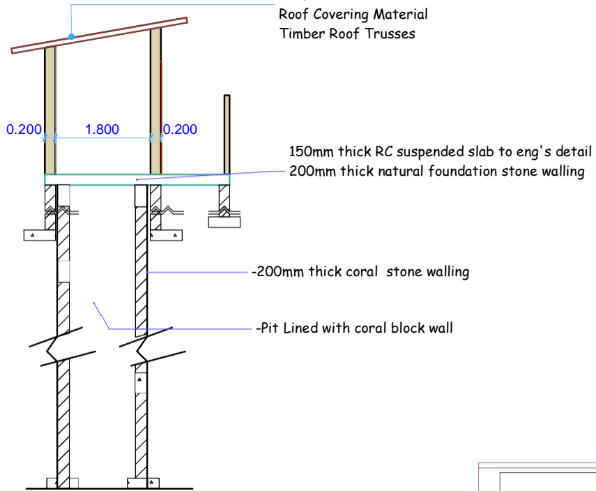
SECTION M-M
