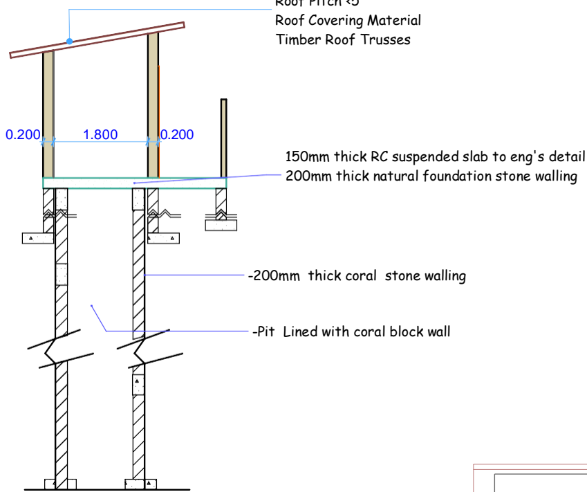
SECTION M-M
