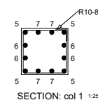
SECTION: col 1 1:25
