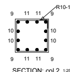
SECTION: col 2 1:25
