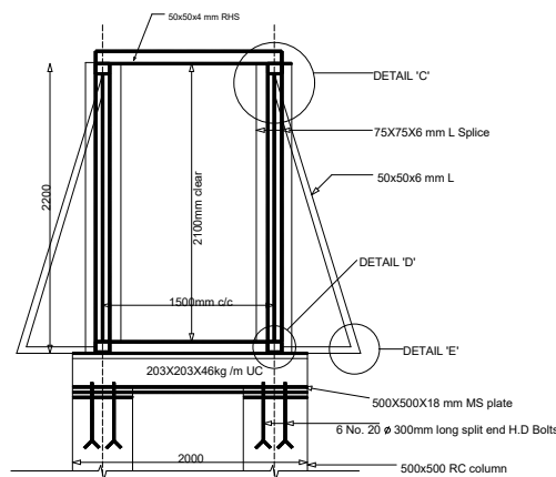
SECTION 'Y-Y' 1:20
