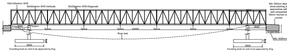
FOOTBRIDGE SAFETY CAGE AND SUPPORT DETAILS 1:100
