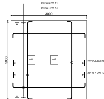
COLUMN BASE DETAILS 1:50
