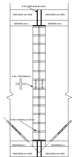
TYPICAL SPLICE DETAIL 1:10
