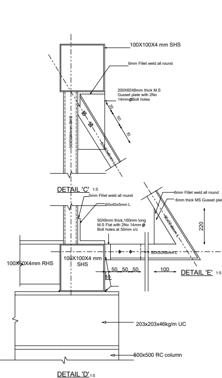
DETAIL 'D' 1:5
