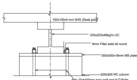
SECTION 'X-X' (ANCHORAGE PLATE DETAIL) 1:20
