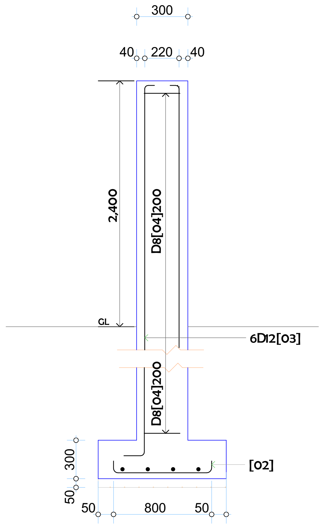
TYPICAL 350X350MM R.C COLUMN R.C DETAILS. 1:25
