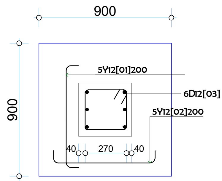
TYPICAL BASE 300x900x900 R.C DETAILS 1:25
