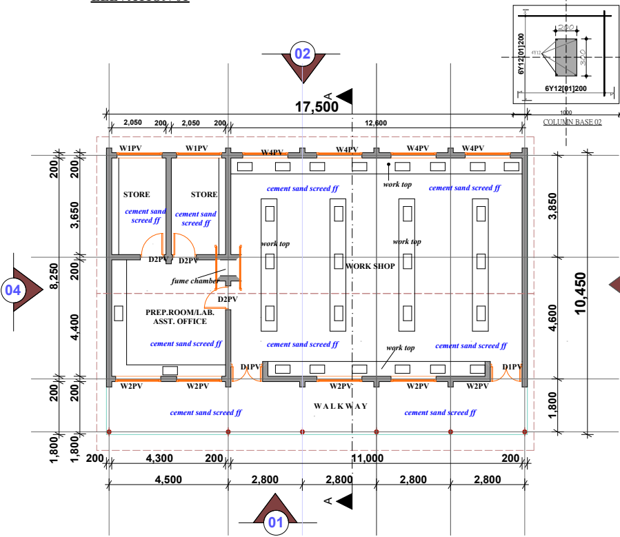
FLOOR PLAN LAYOUT
