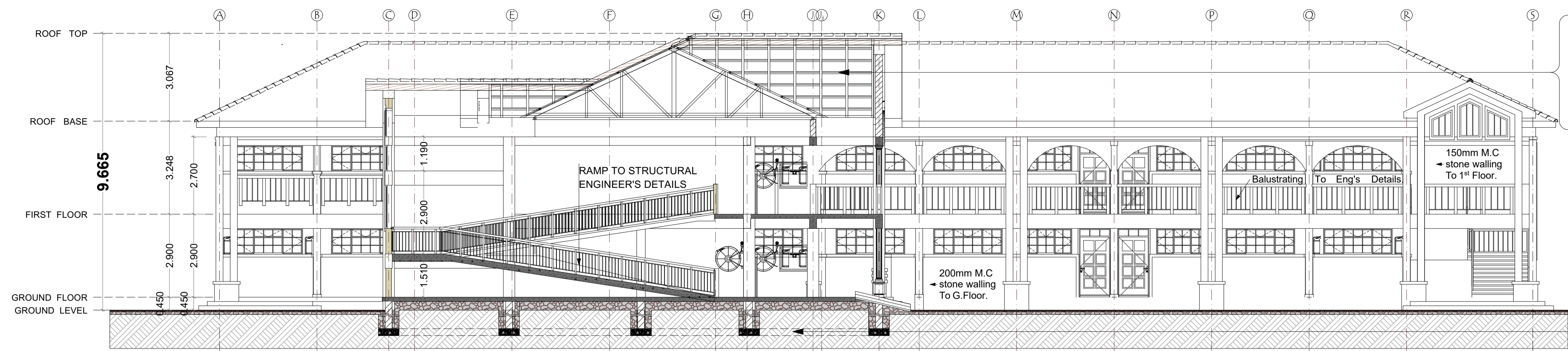
SECTION S-02 SCALE 1:100
