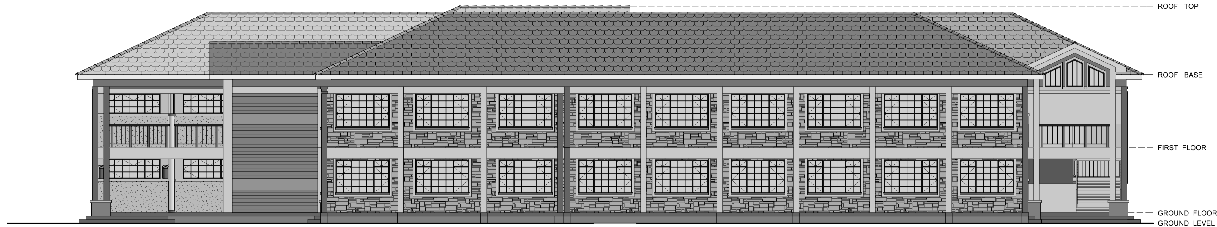
02 ELEVATION SCALE 1:100
