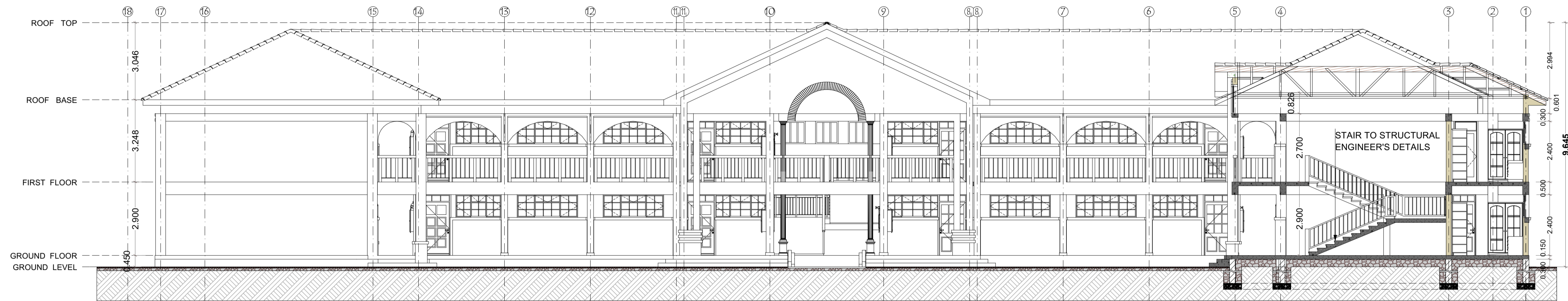
SECTION S-02 SCALE 1:100
