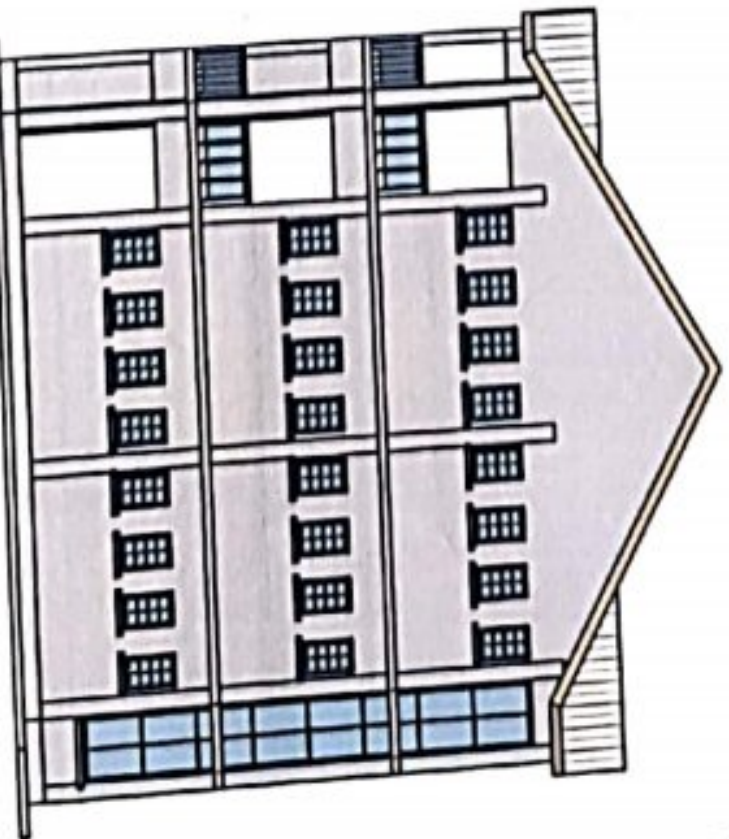
EAST ELEVATION
