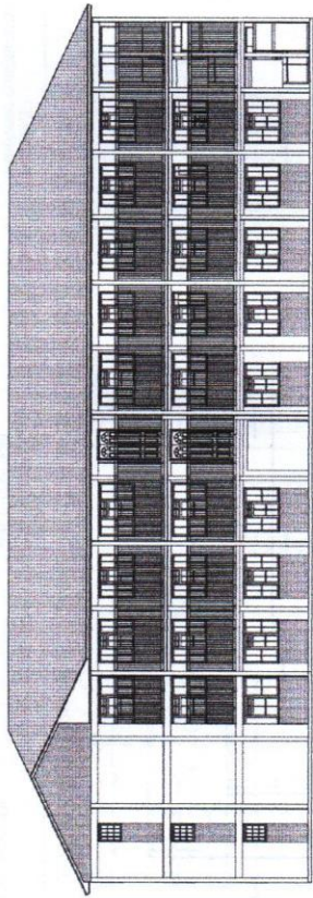
ELEVATION B-02 DETAILS 1:100
