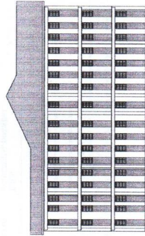
ELEVATION B-02 DETAILS 1:100
