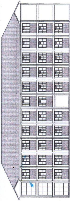
ELEVATION B-04 DETAILS 1:100
