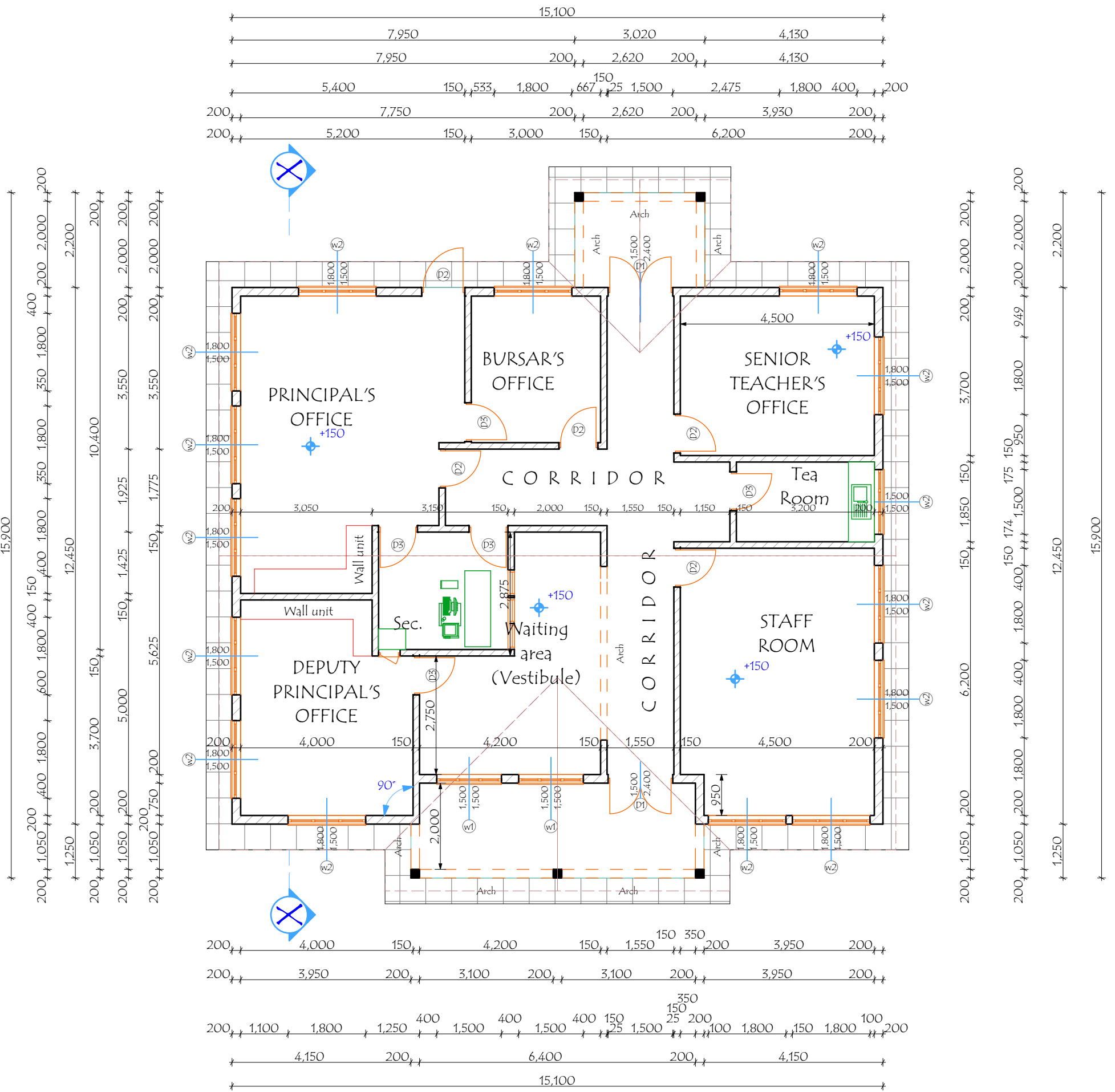
FLOOR PLAN
