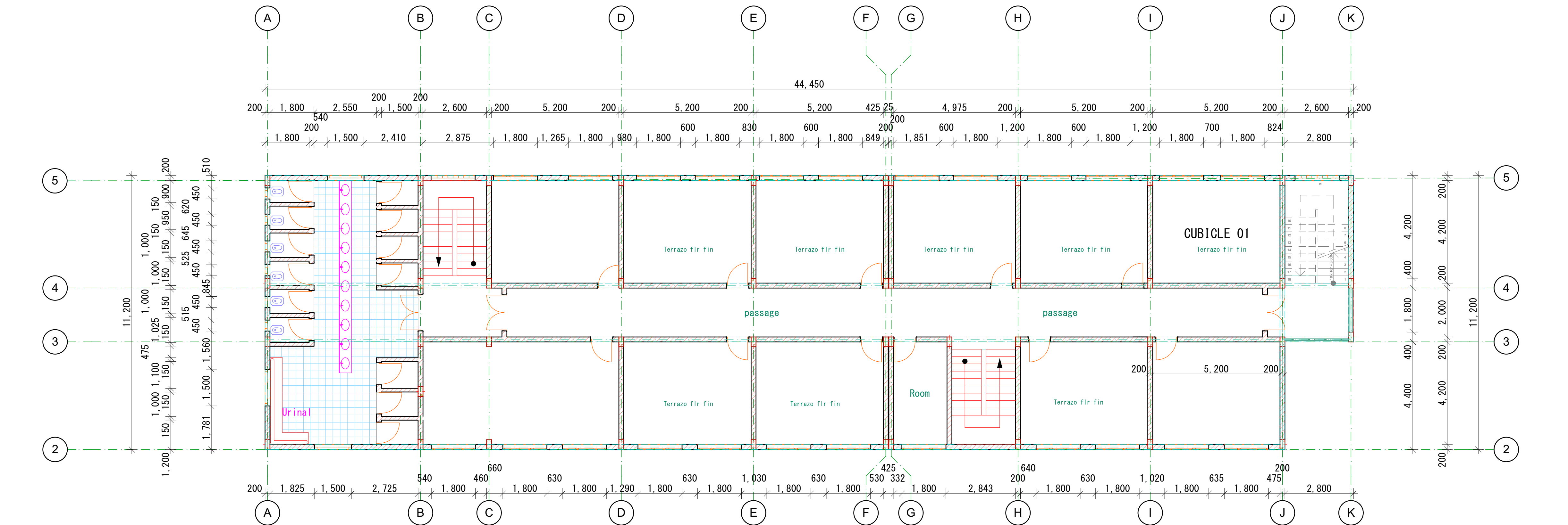
TYPICAL 1 ST 2 ND 3 RD FLOOR LAYOUT PLAN
