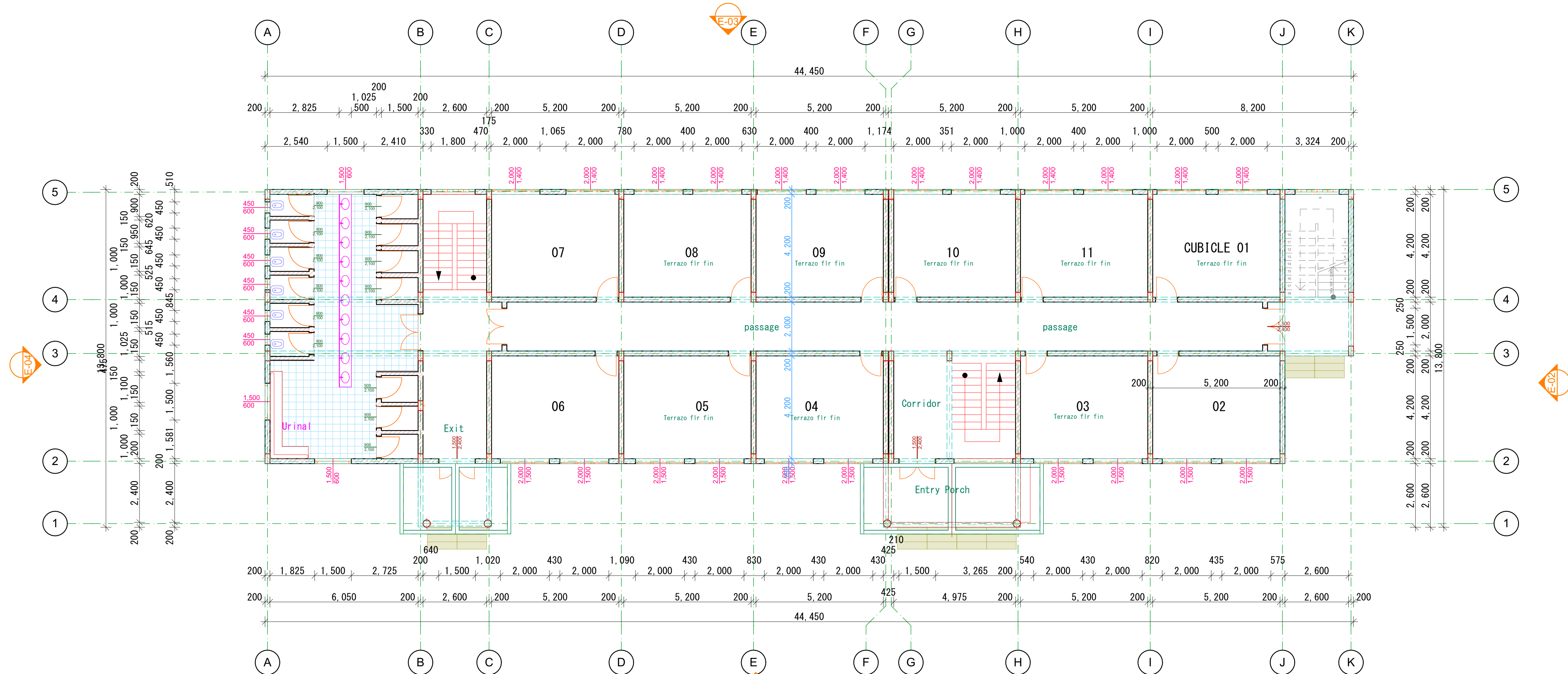
GROUND FLOOR PLAN LAYOUT
