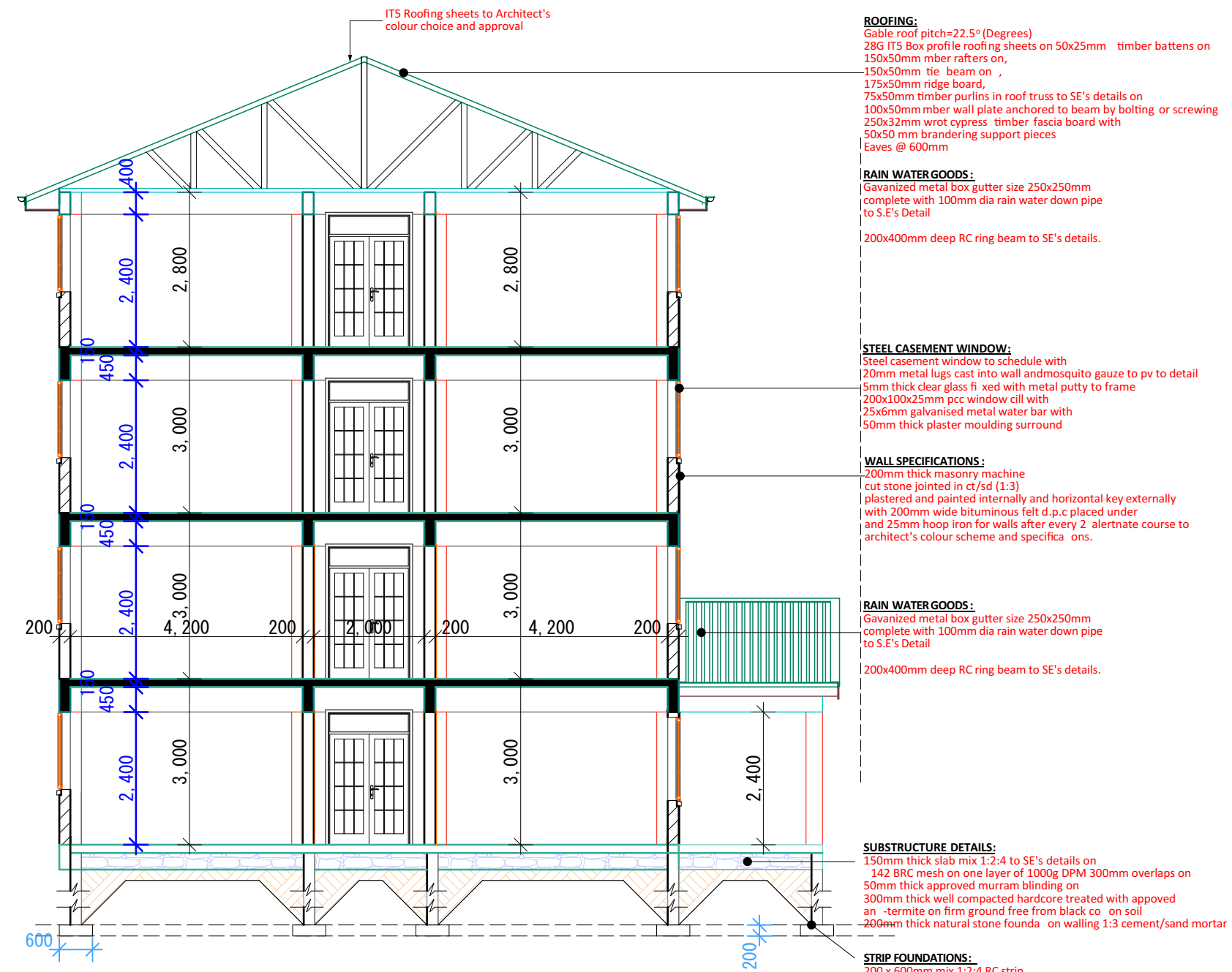
BUILDING SECTION
