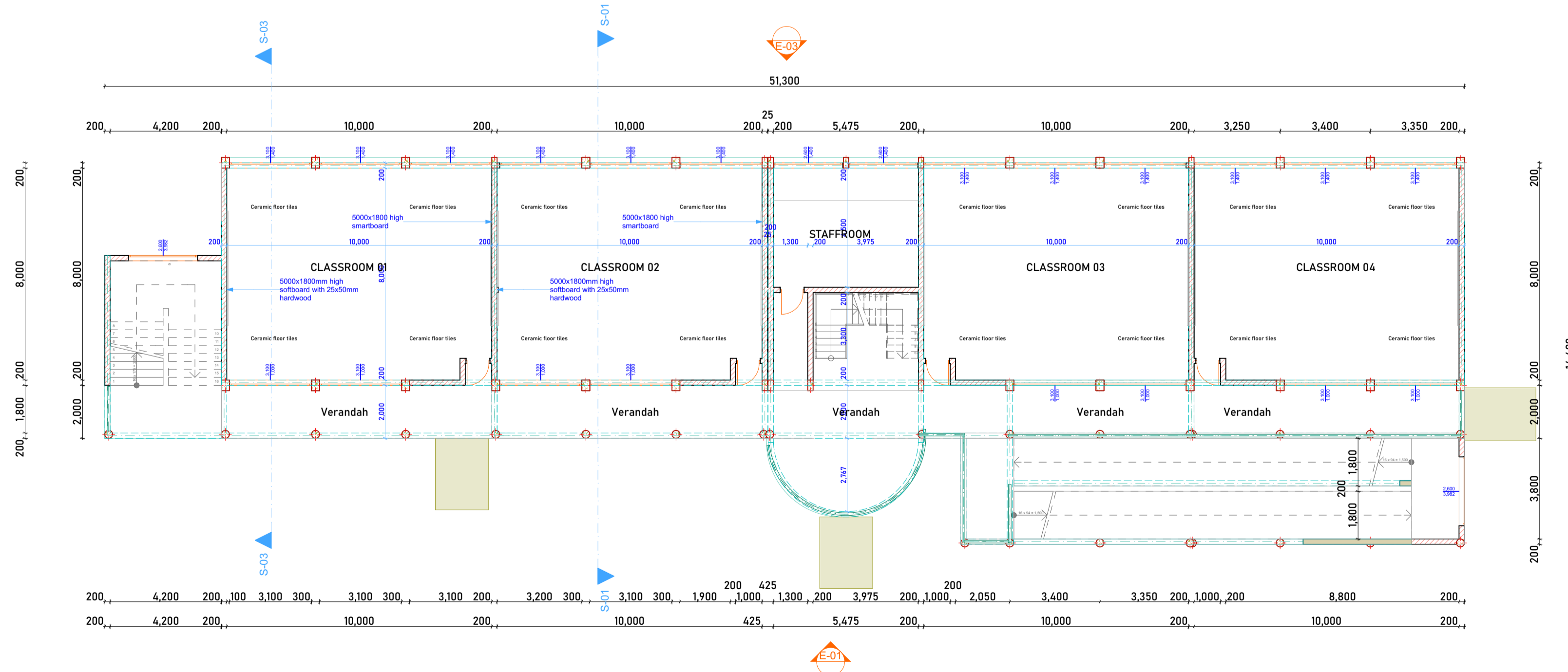
TYPICAL GROUND AND FIRST FLOOR PLAN
