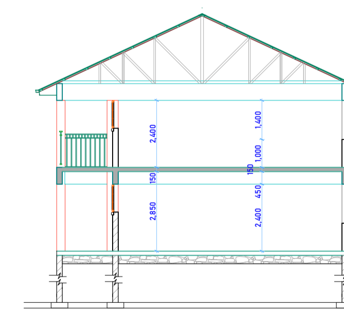
Building Section
