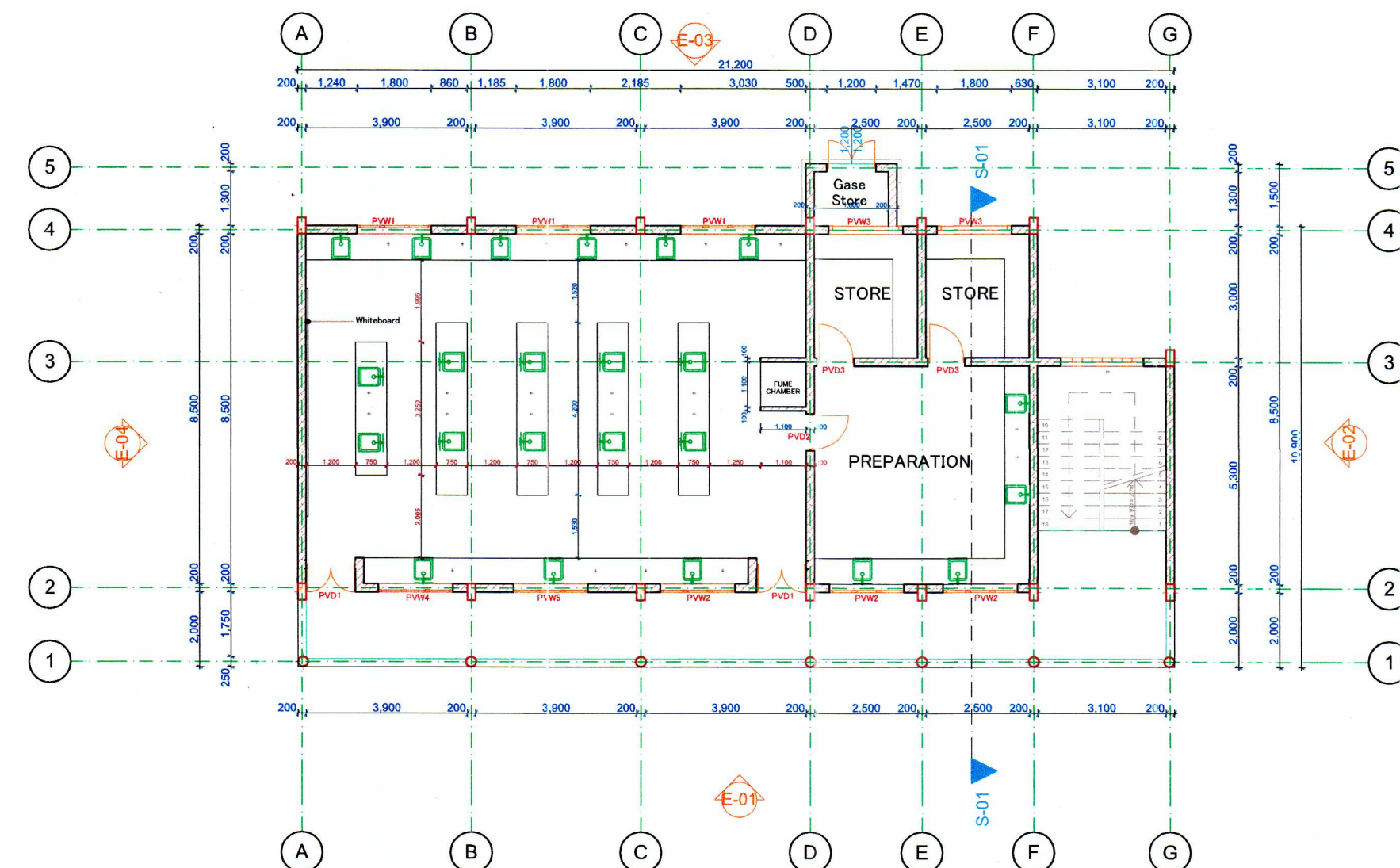
GROUND & 1ST FLOOR PLAN LAYOUT
