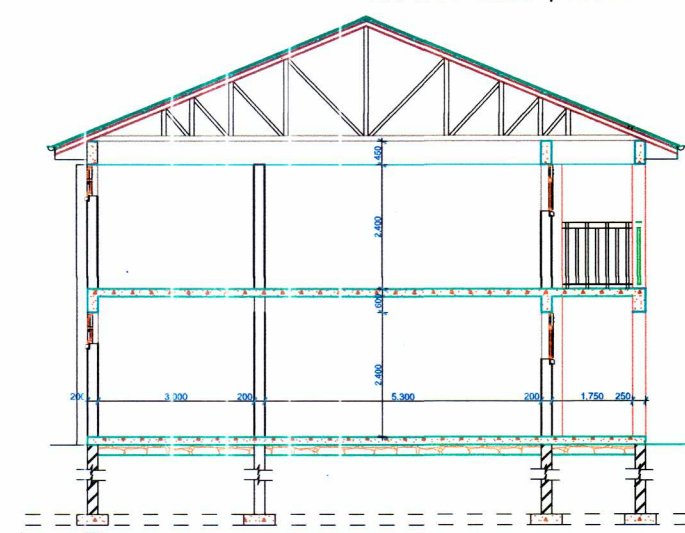
BUILDING SECTION
