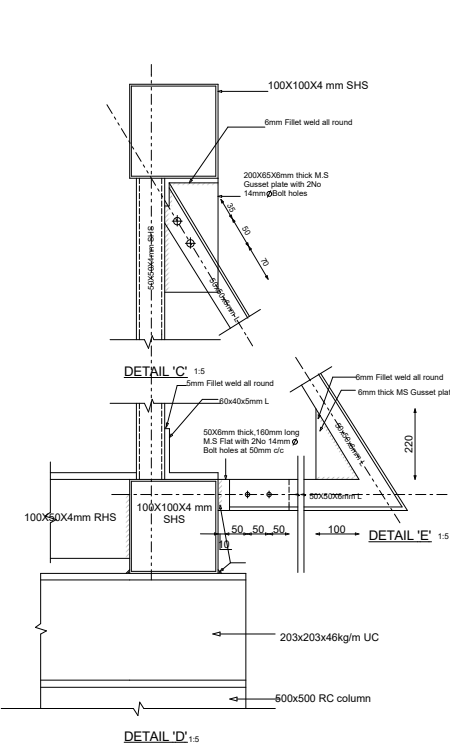
DETAIL 'D' 1:5
