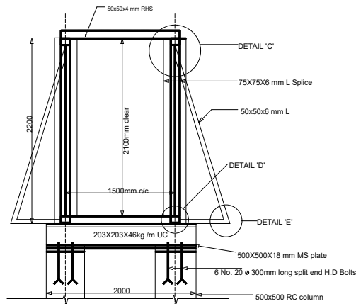
SECTION 'Y-Y' 1:20
