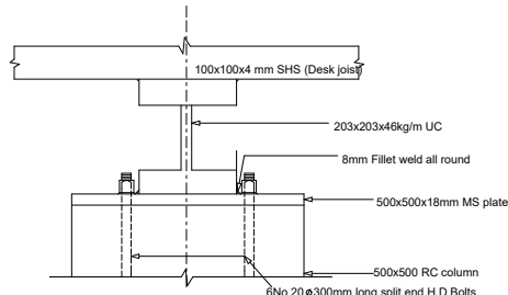
SECTION 'X-X' (ANCHORAGE PLATE DETAIL) 1:20
