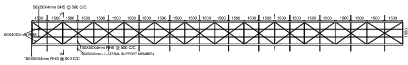
DECKING BEARERS AND WIND BRACING BOTTOM VIEW 1:100
