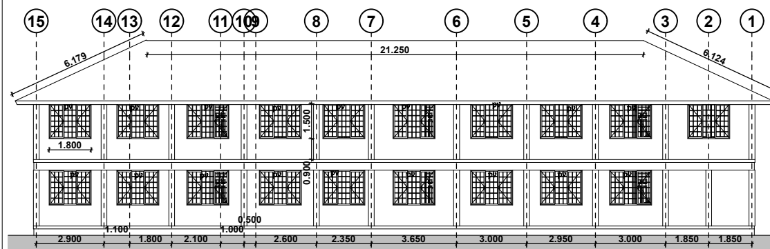
ELEVATION 03
