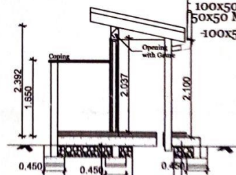
SECTION 02-02 SCALE 1:100
