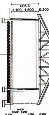
SECTION 01-01
