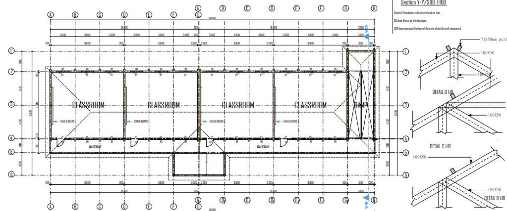
FIRST FLOOR PLAN LAYOUT 1:100
