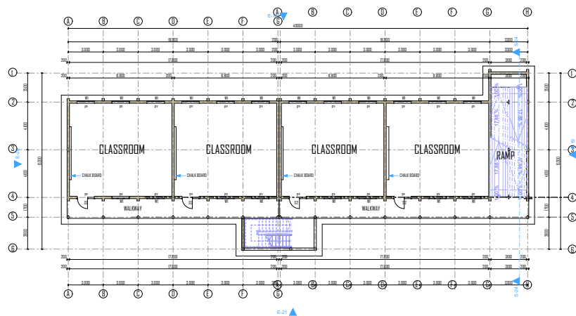
GROUND FLOOR PLAN LAYOUT 1:100
