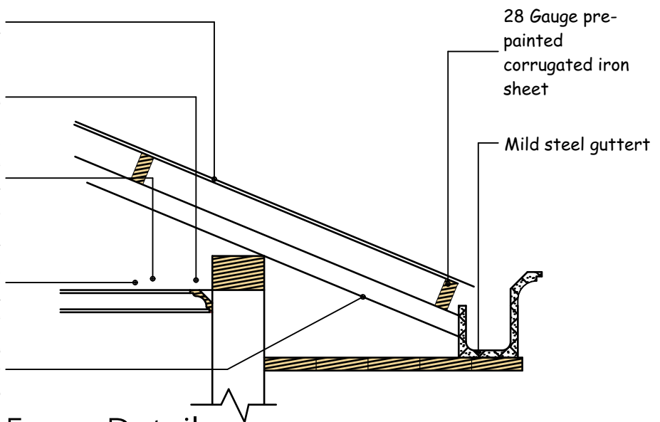
Eaves Details
