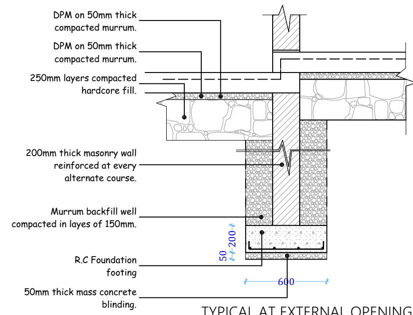
TYPICAL AT EXTERNAL OPENING FOUNDATION WALLS SCALE 1:25
