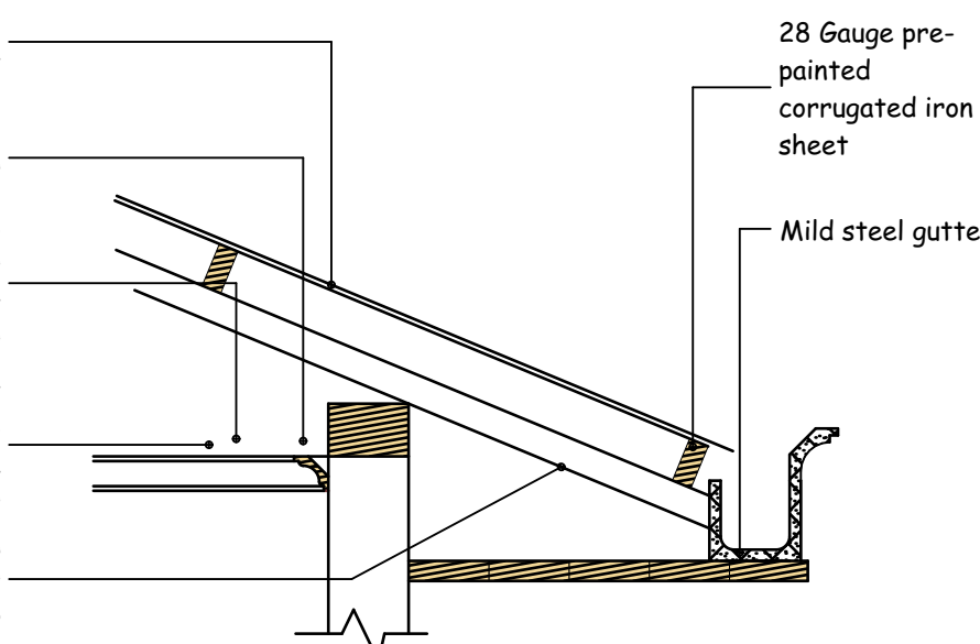
Eaves Details
