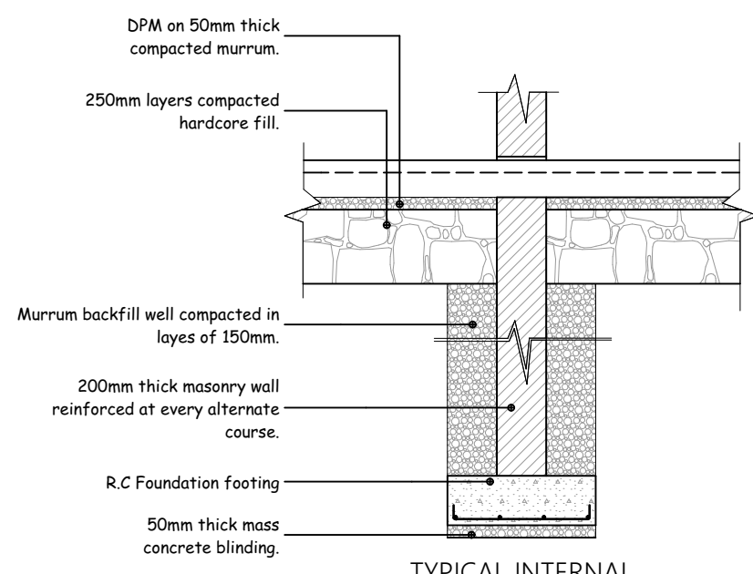
TYPICAL INTERNAL FOUNDATION WALLS SCALE 1:25
