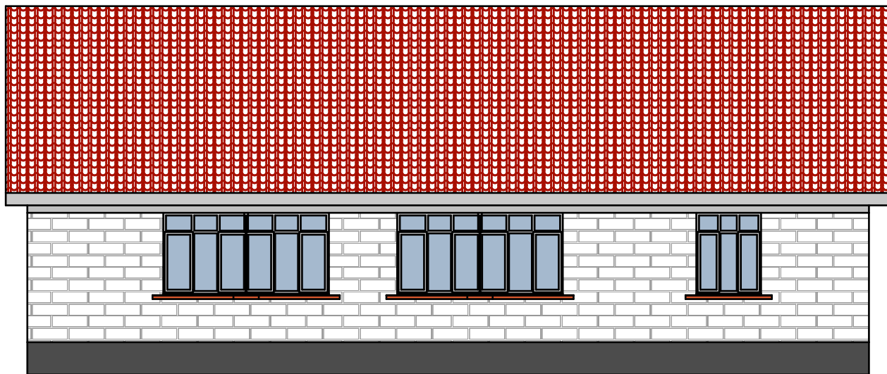
ELEVATION 03
