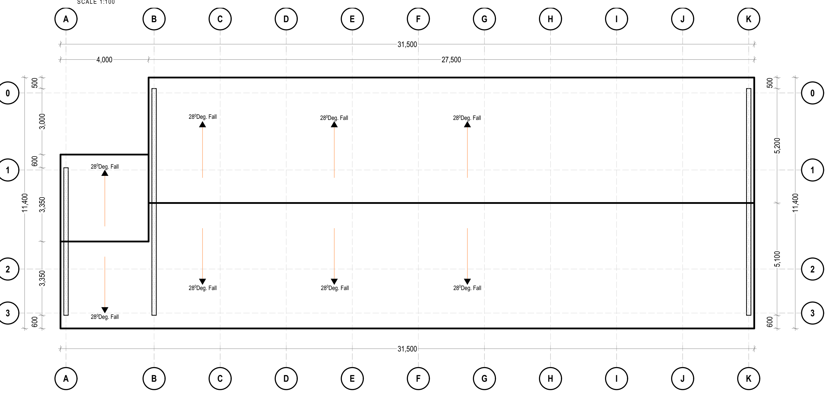
Roof Plan Layout
