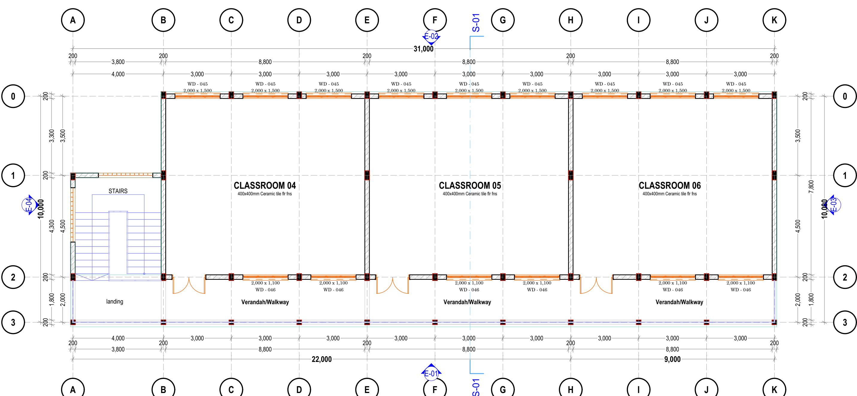
1ST FLOOR PLAN
