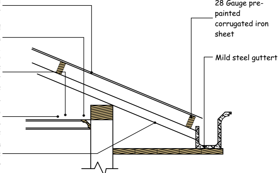
Eaves Details
