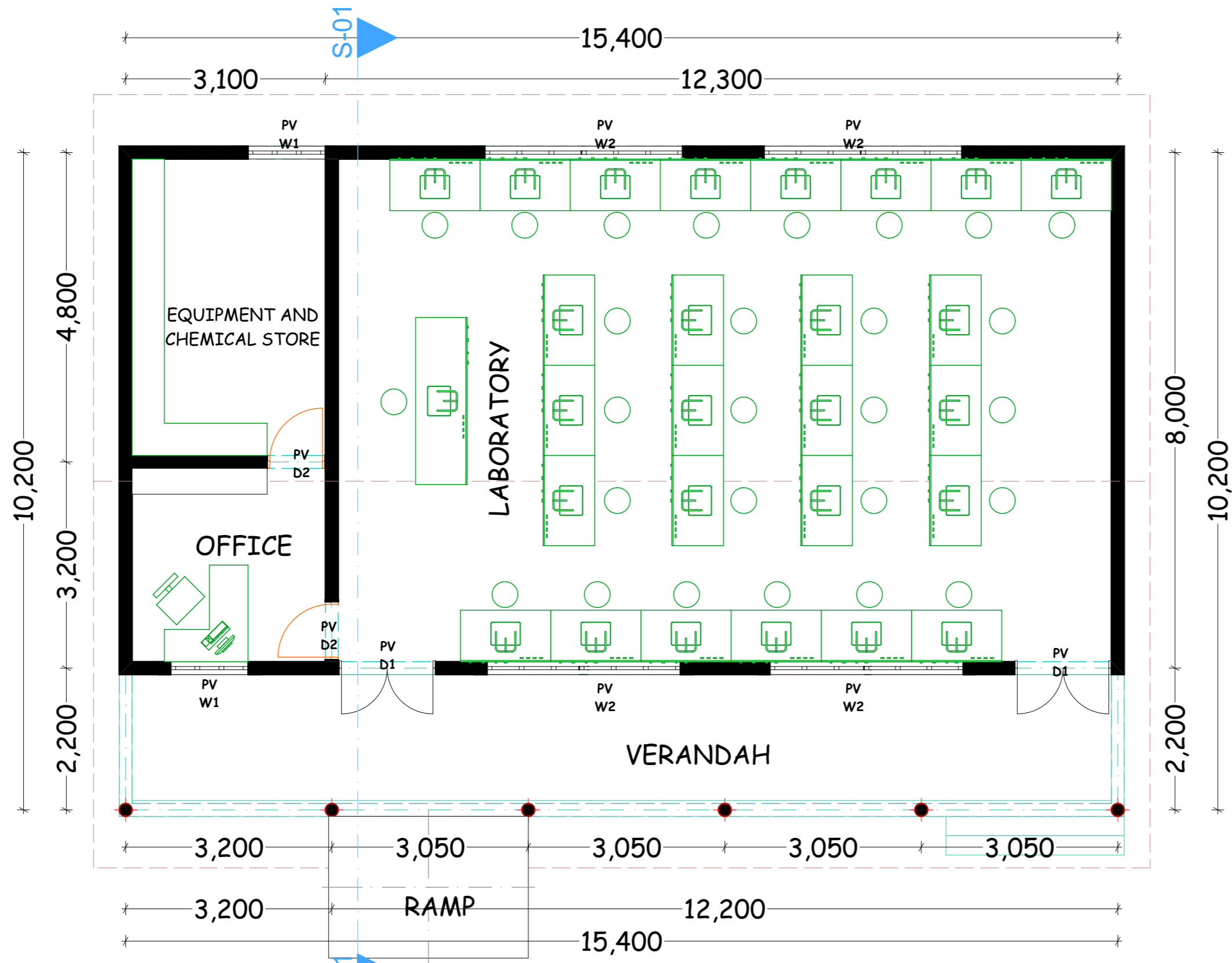
FLOOR LAYOUT PLAN
