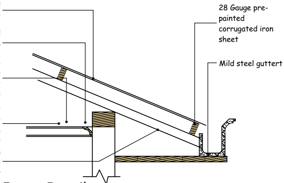
Eaves Details
