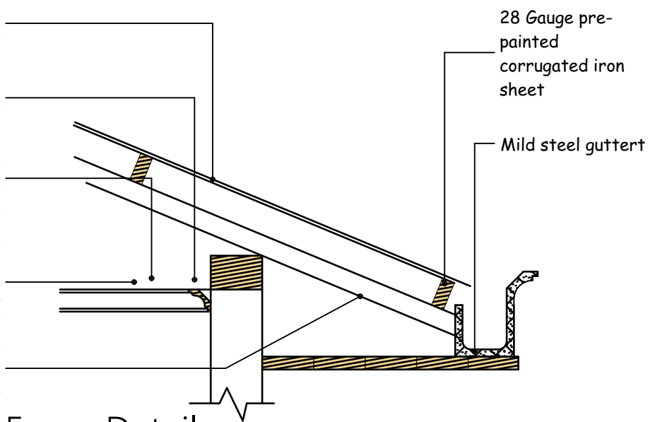
Eaves Details
