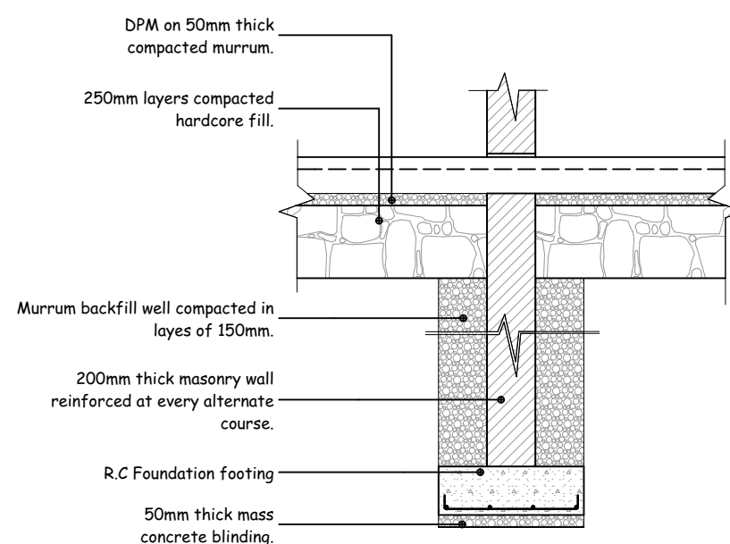
TYPICAL INTERNAL FOUNDATION WALLS
