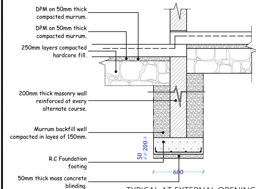
TYPICAL AT EXTERNAL OPENING FOUNDATION WALLS
