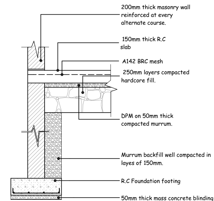
TYPICAL EXTERNAL FOUNDATION WALLS
