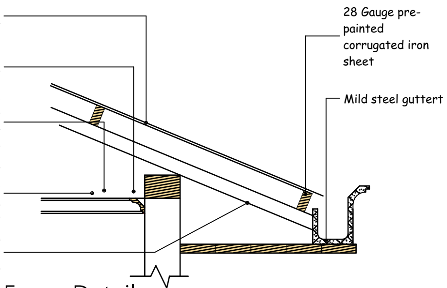
Eaves Details
