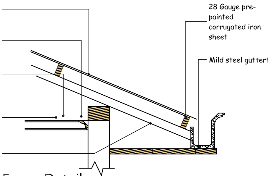
Eaves Details
