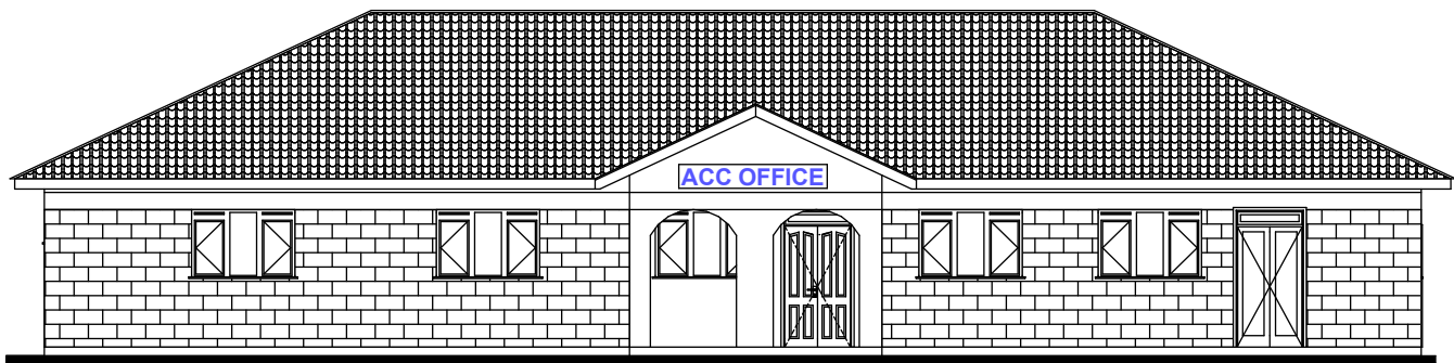
SOUTH ELEVATION
