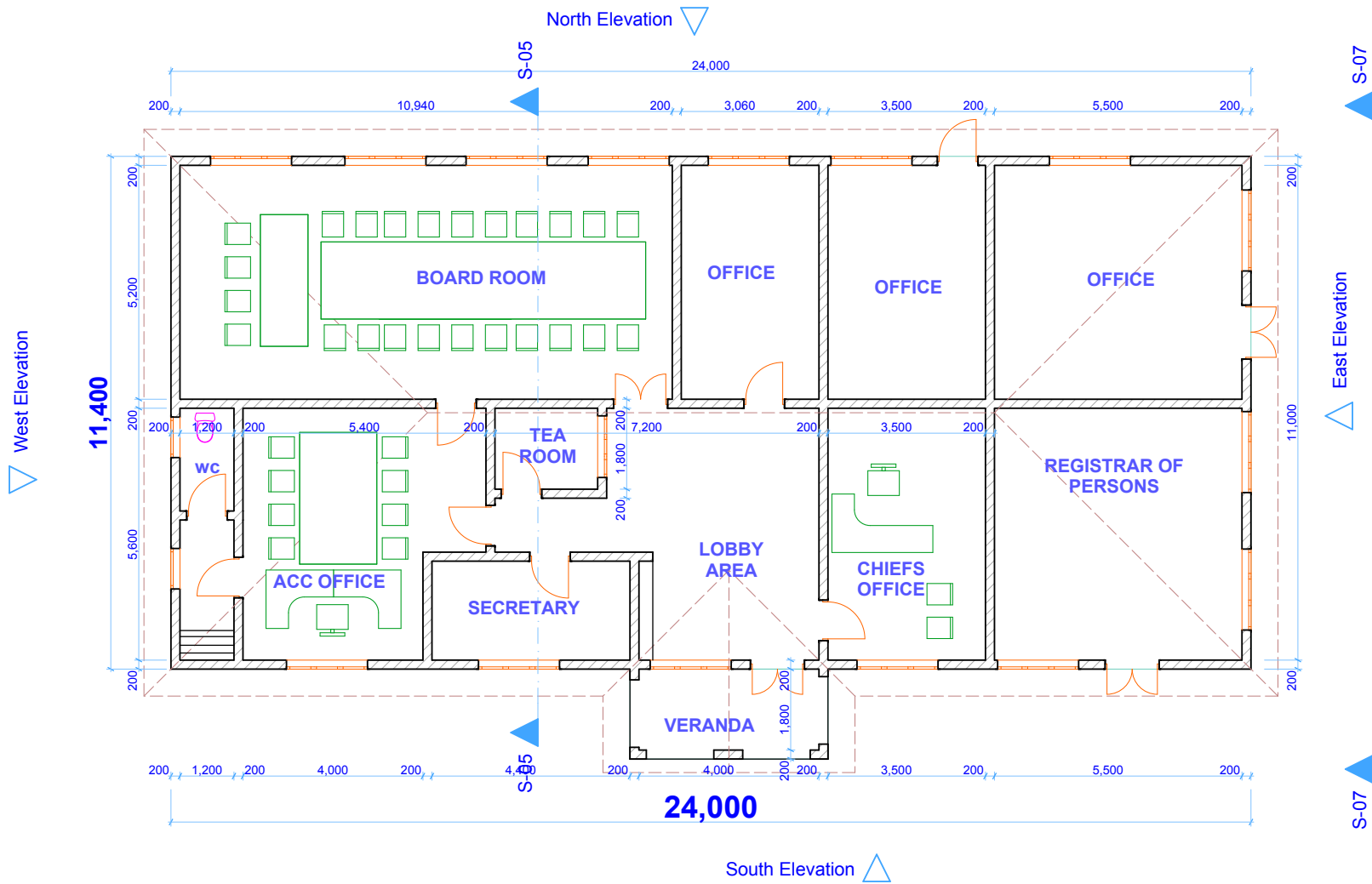
FLOOR PLAN
