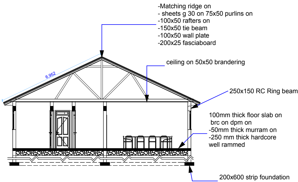
SECTION XX
