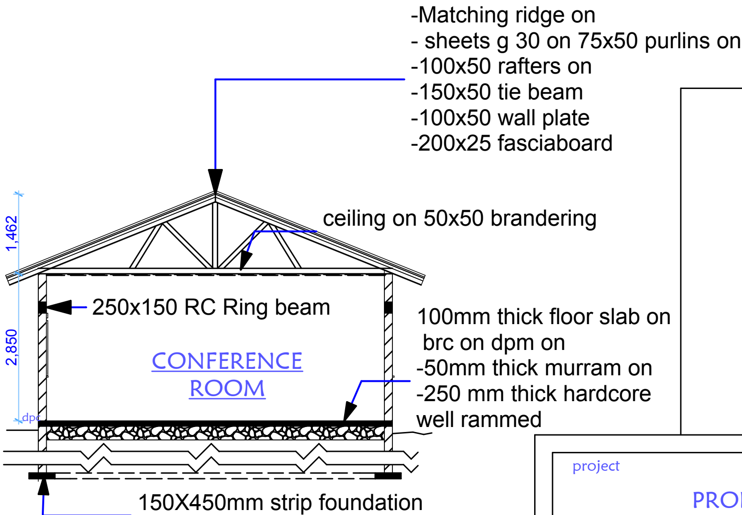
SECTION XX
