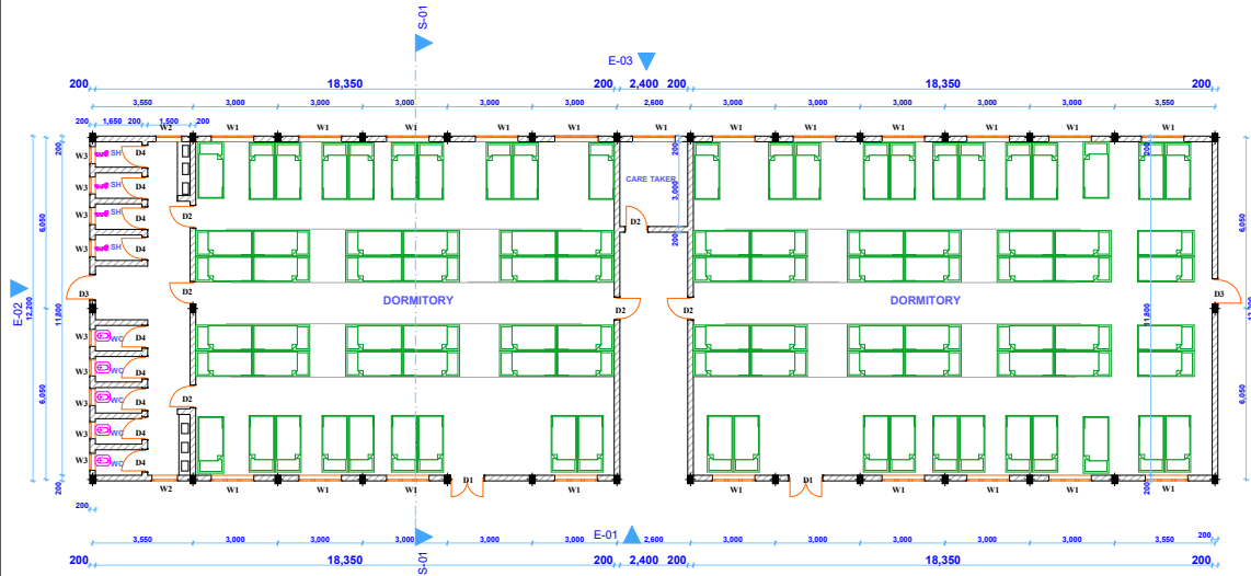
FLOOR PLAN
