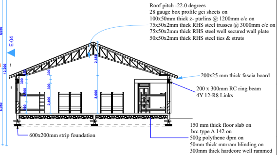
SECTION 01-01
