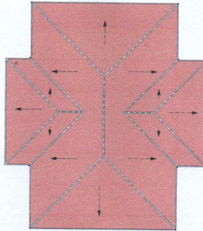
ROOF PLAN
