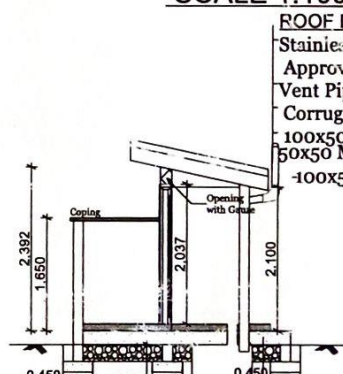
SECTION 02-02 SCALE 1:100
