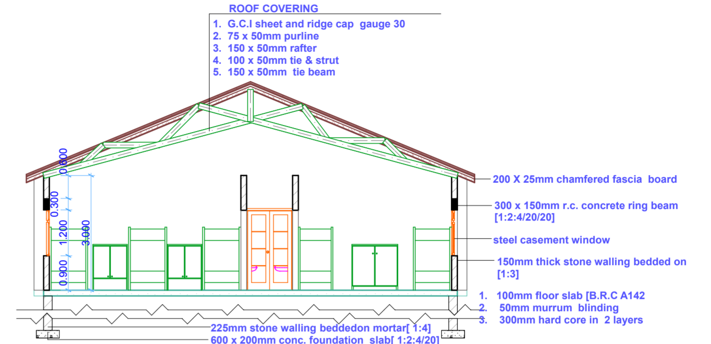
SECTION 01-01
