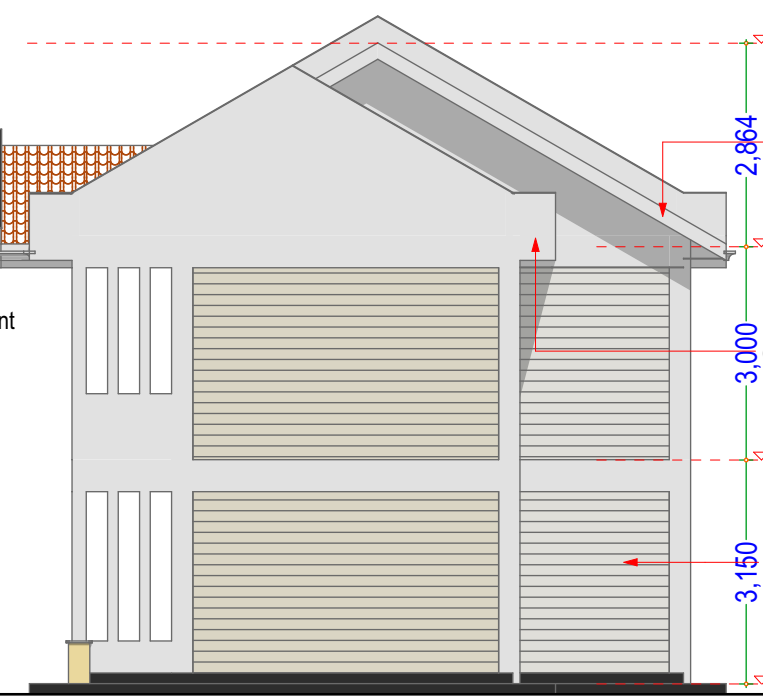
ELEVATION 02 (SCALE 1:100)
