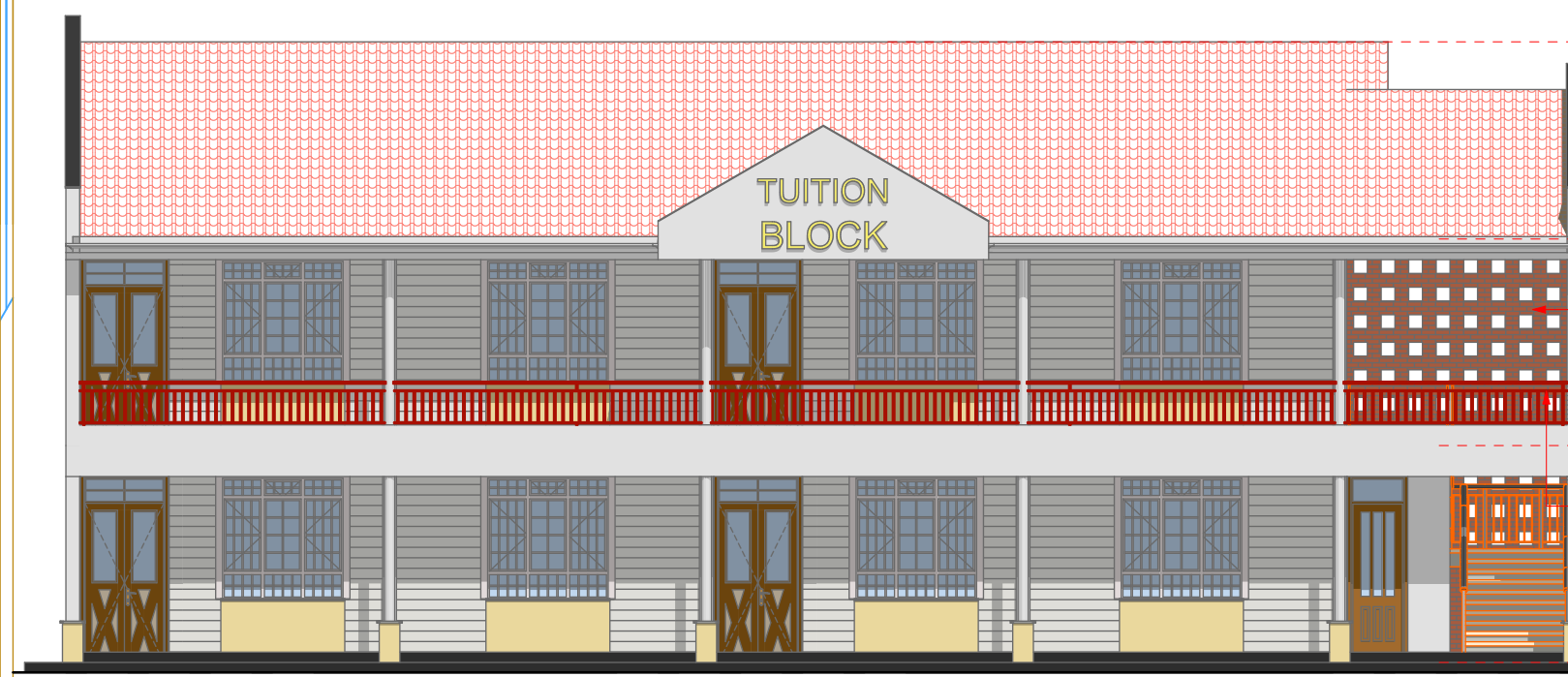
ELEVATION 01 (SCALE 1:100)
