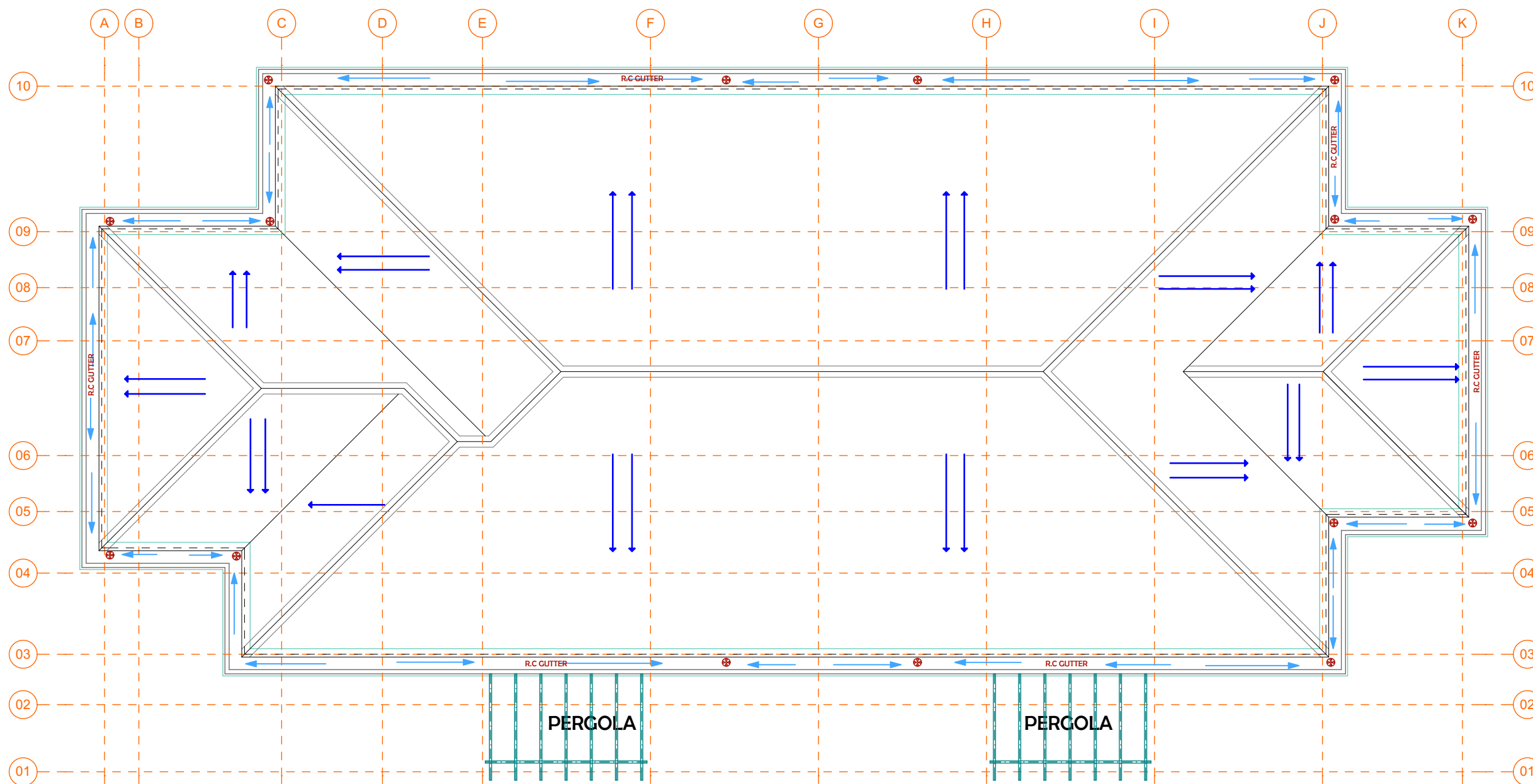
ROOF LAYOUT
