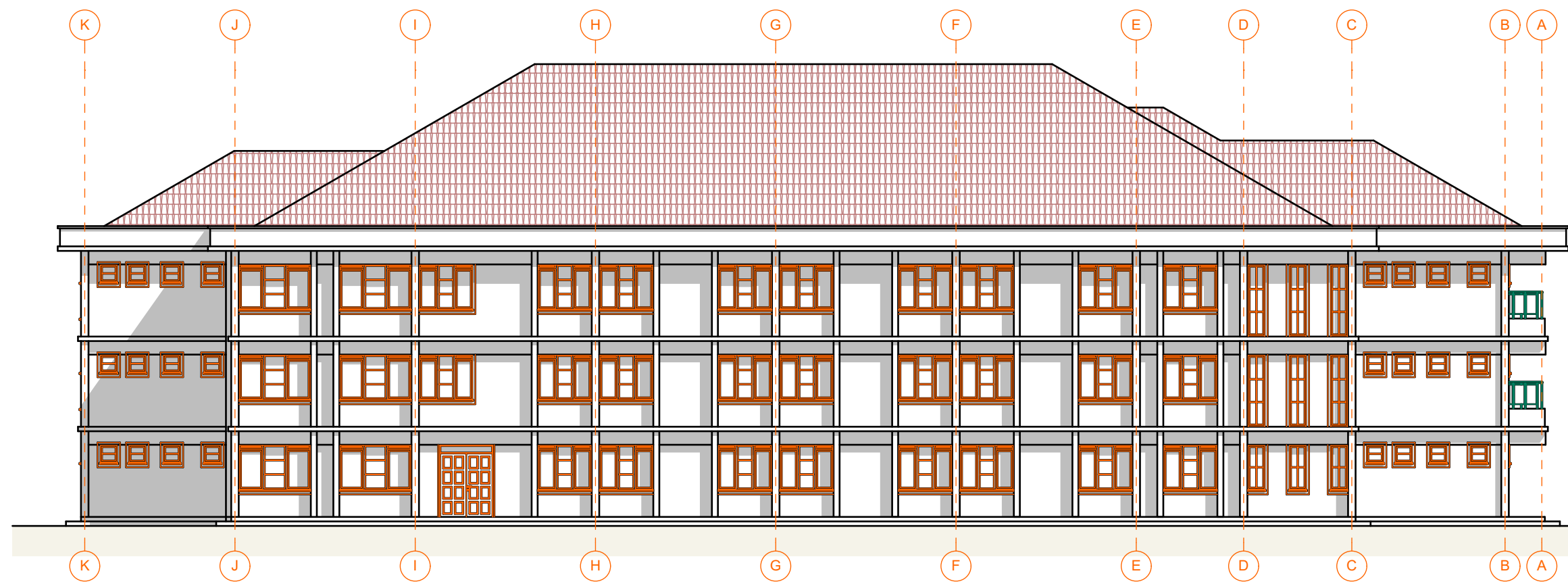
ELEVATION E-02
