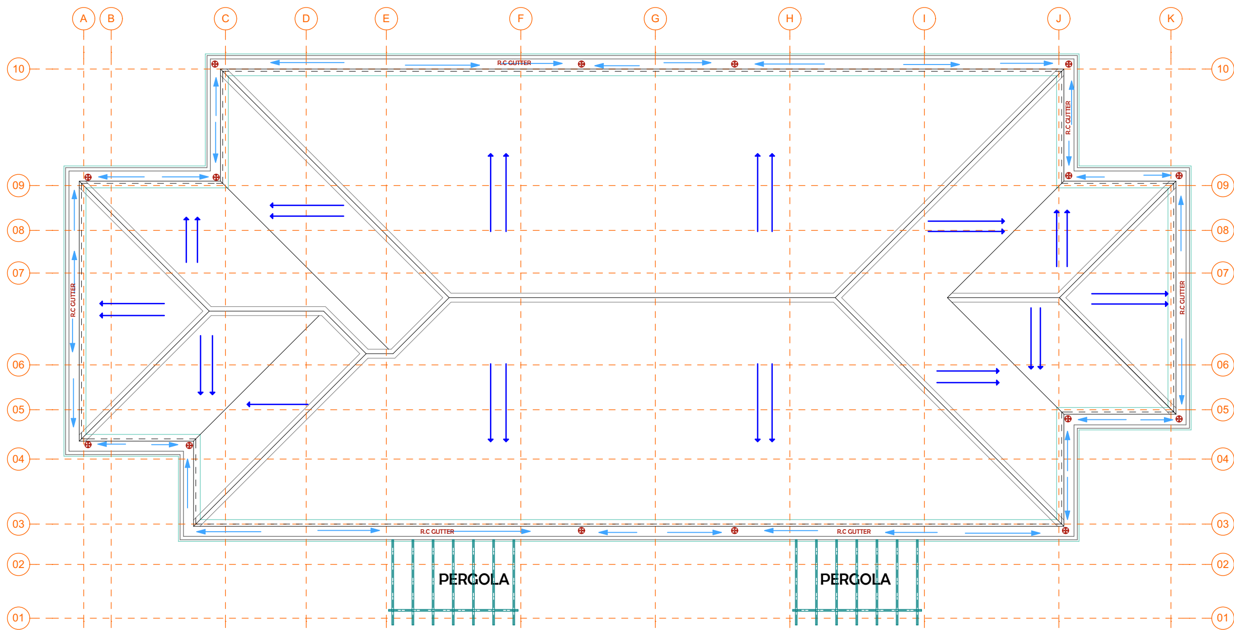
ROOF LAYOUT
