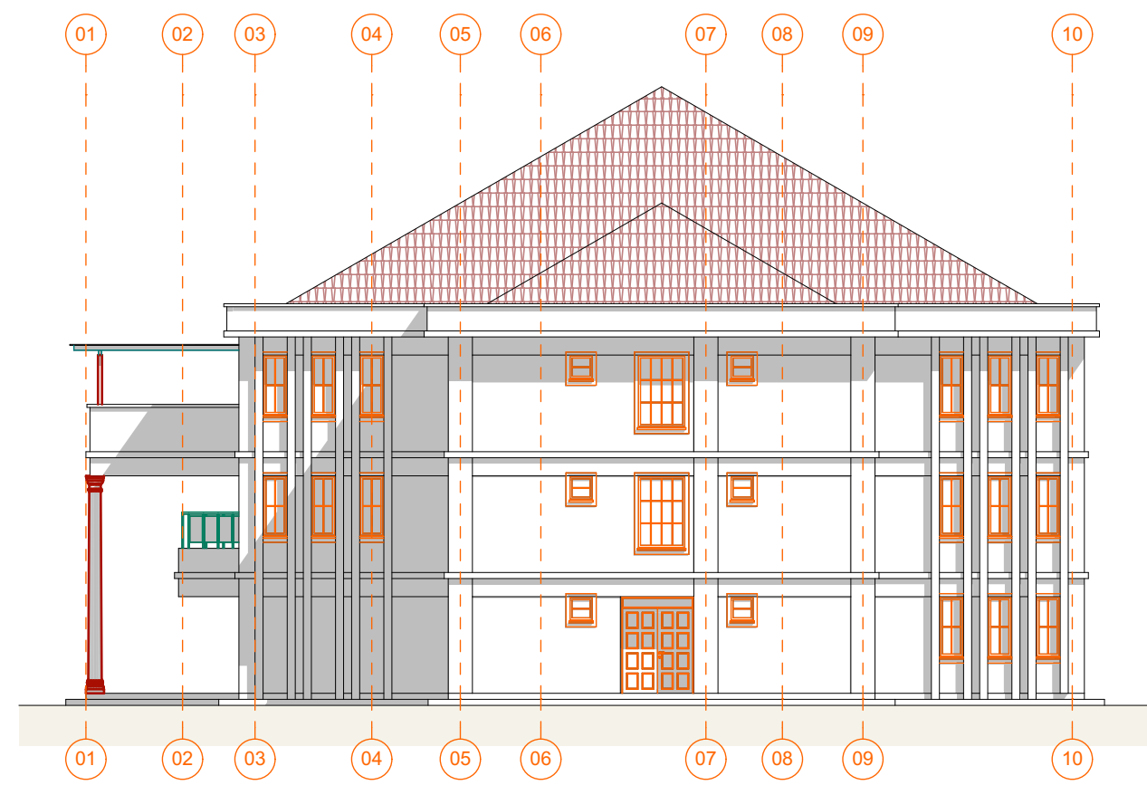
ELEVATION E-04
