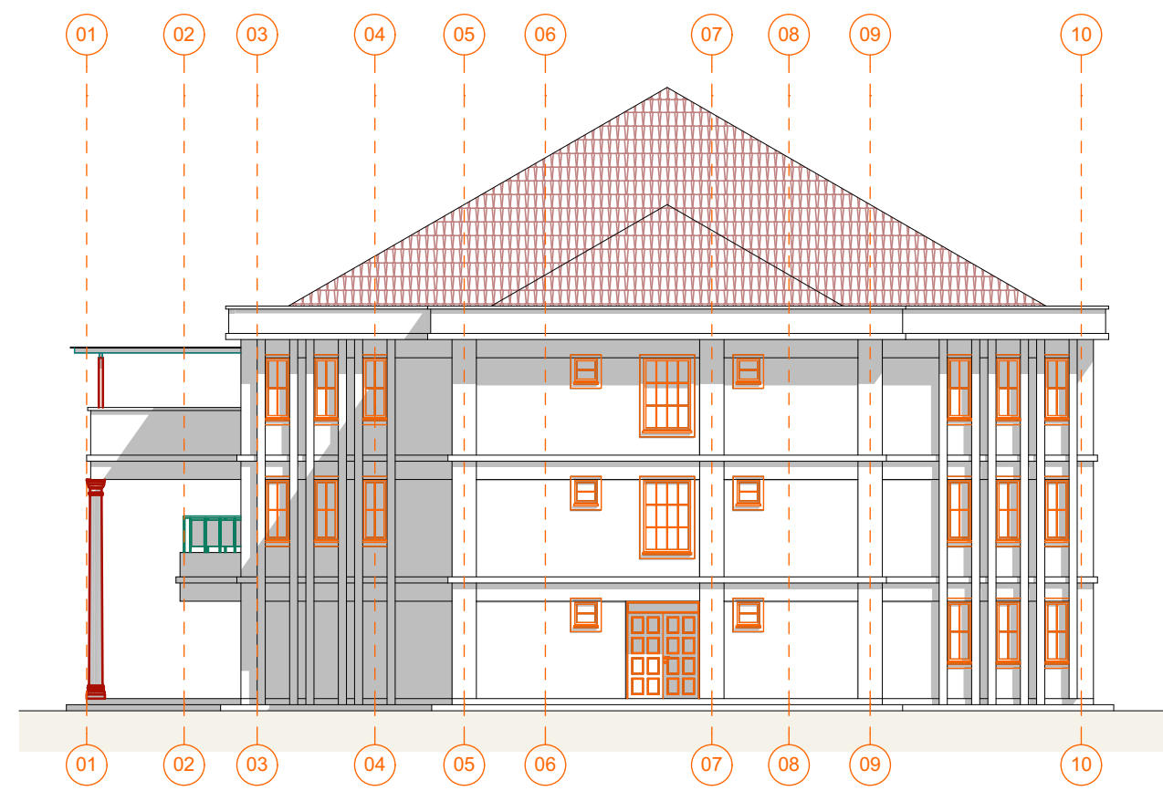
ELEVATION E-04
