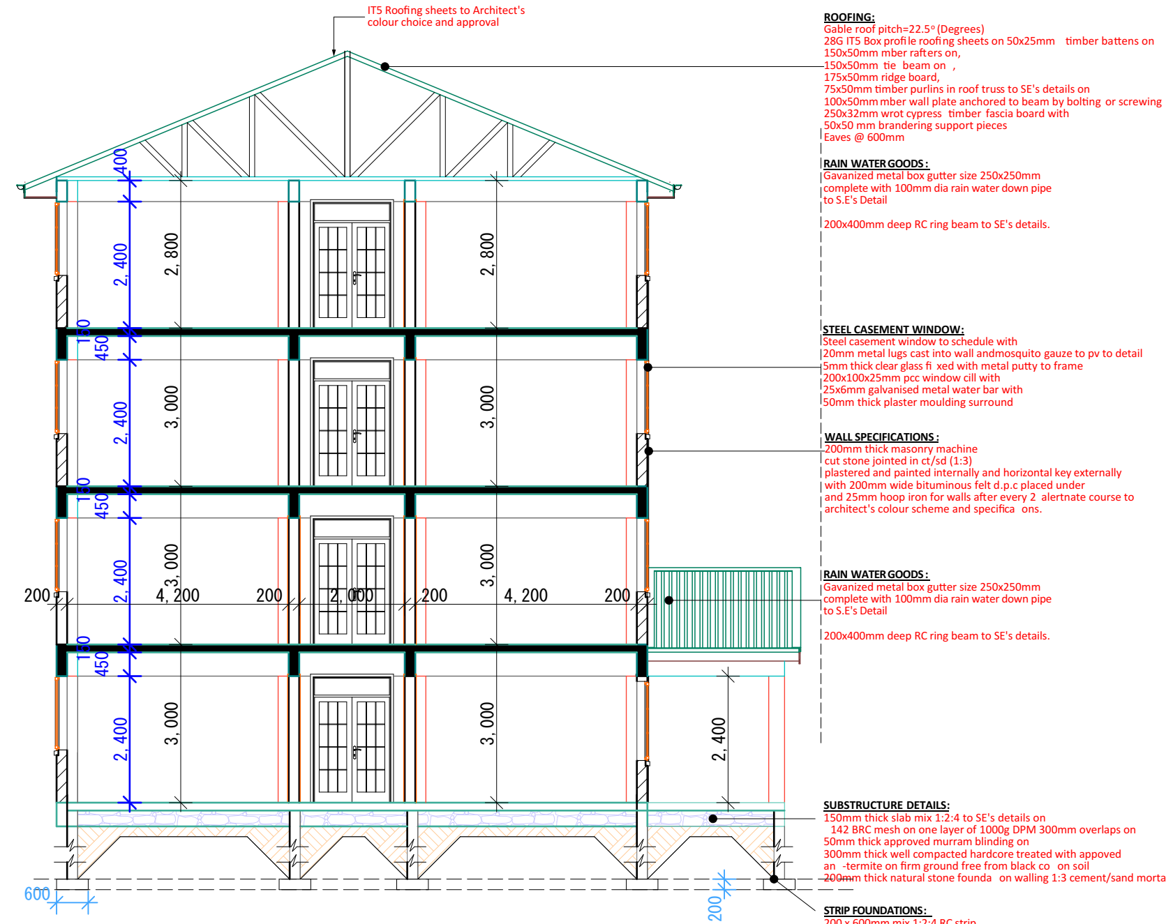
BUILDING SECTION
