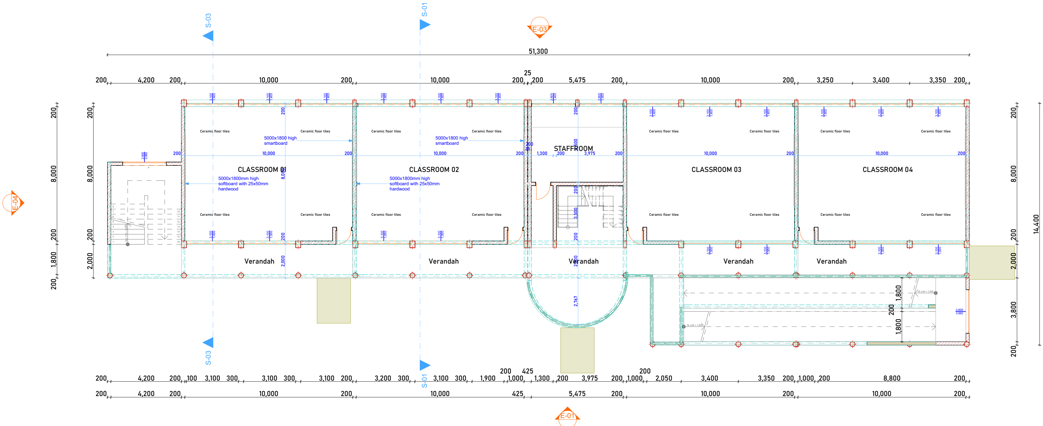
TYPICAL GROUND AND FIRST FLOOR PLAN
