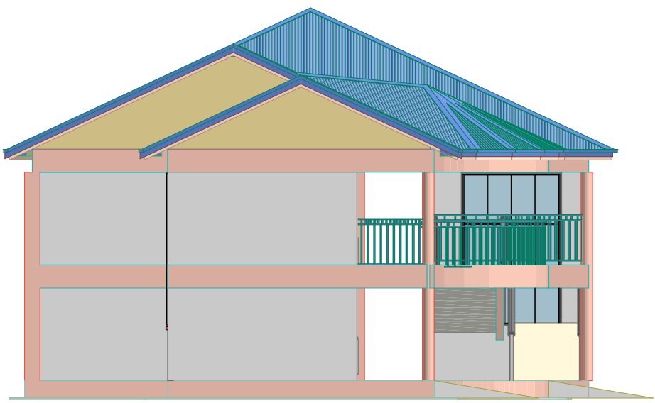
LEFT HANDSIDE ELEVATION
