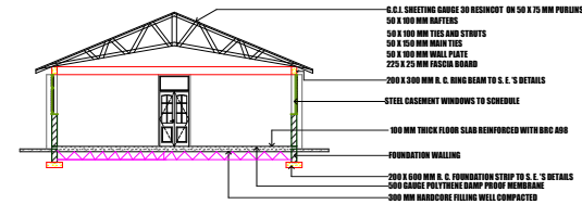
SECTION X-X
