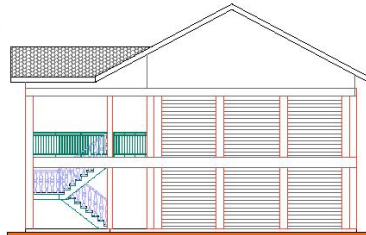
ELEVATION E-01
