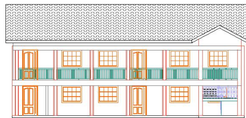
ELEVATION E-04
