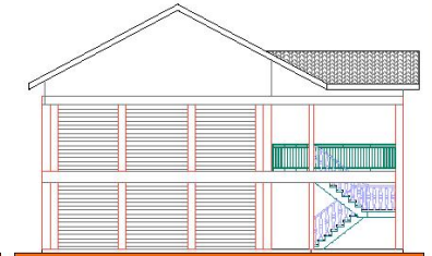
ELEVATION E-03
