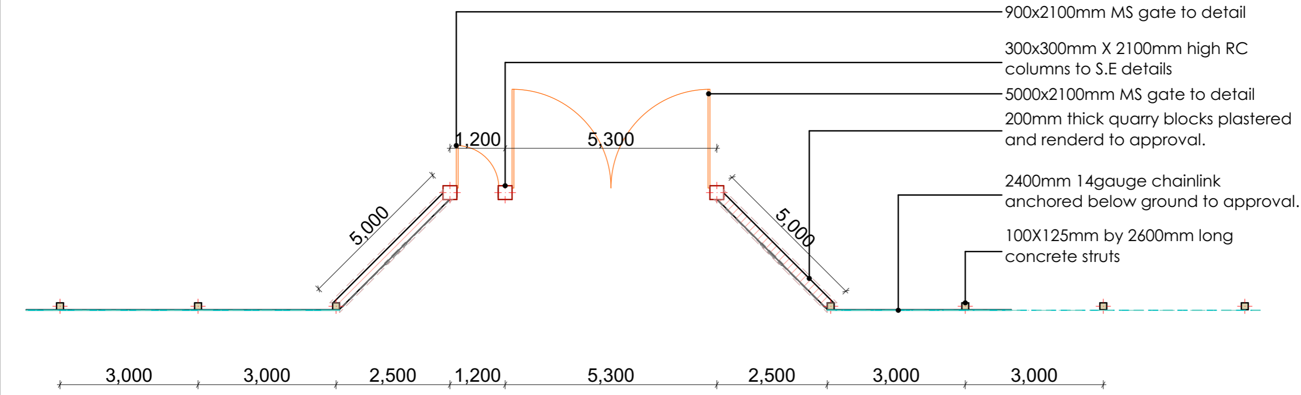
LAYOUT PLAN Scale 1:100
