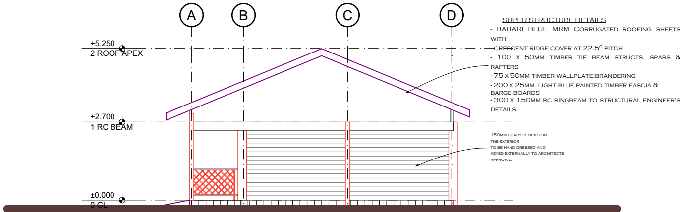
ELEVATION E-2
