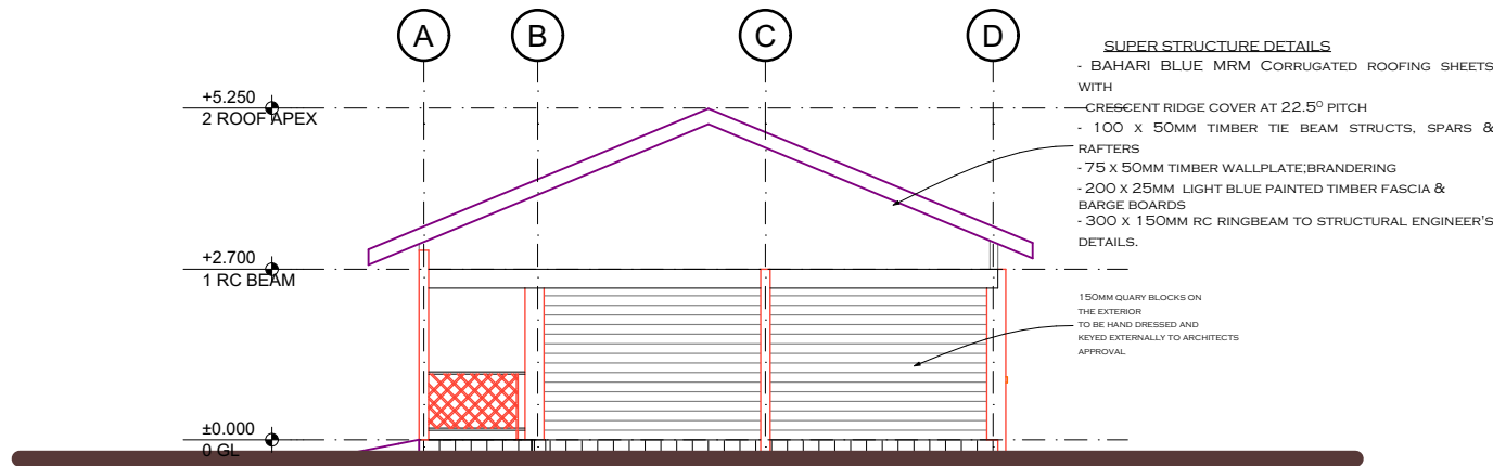
ELEVATION E-2
