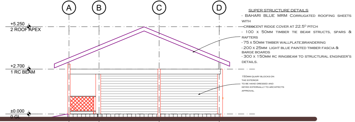
ELEVATION E-2 scale 1:100
