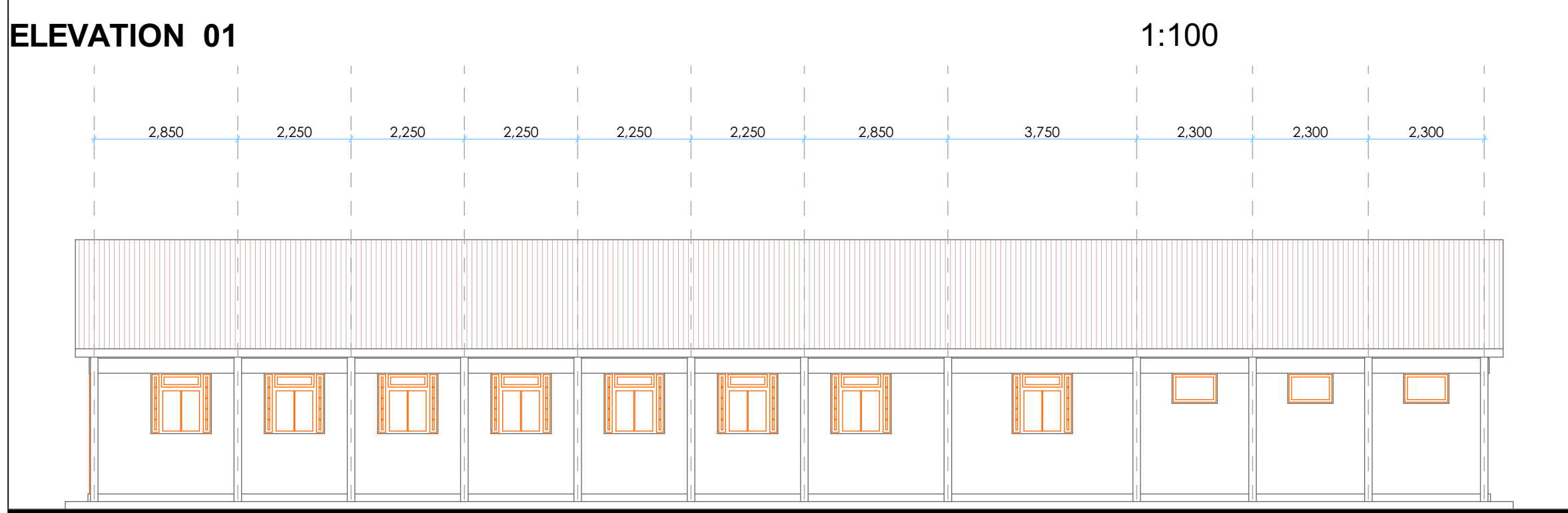
ELEVATION 03
